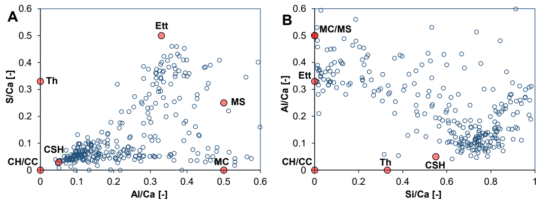
Figure 3.2: S/Ca-ratio as a function of the Al/Ca-ratio (left) and Al/Ca-ratio as a function of the Si/Ca-ratio (right). CH = portlandite, CC = calcite, CSH = calcium-silicate-hydrate, Th = thaumasite, Ett = ettringite, MS = monosulphate, MC = monocarbonate. Front of home, rising blocks.
