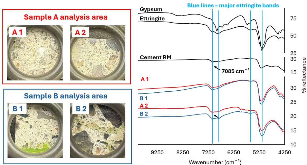
Figure 3.4: NIR spectra for gypsum, ettringite and cement compared to locations on concrete samples, sample areas (9 mm diameter) A and B.
