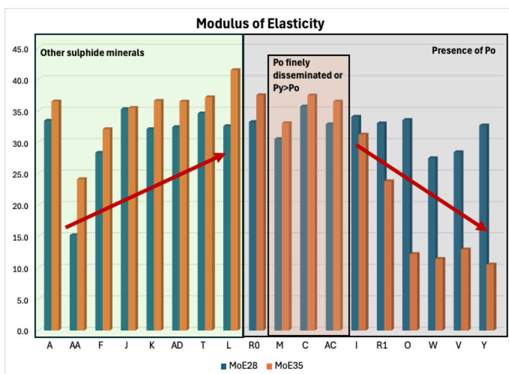
Figure 4.2: MoE values of control concrete specimens (blue bars) vs concrete specimens subjected to electrochemical testing (orange bars).
