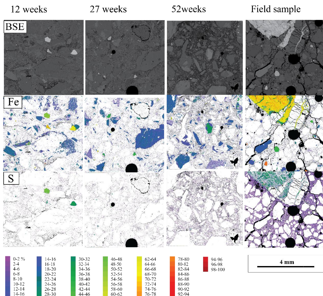
Figure 1: AM field mapping of the AMBT samples and the concrete field sample. Images were acquired with a 2 \mu\text{m} step size. Elemental heat mapping of Fe and S using 2% concentration intervals
