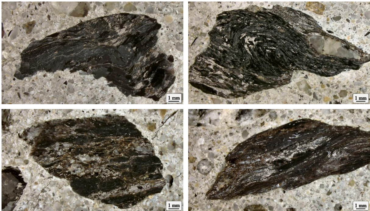
Figure 2: Examples of the reactive, pyrrhotite-bearing A/W schist coarse aggregate particles.
