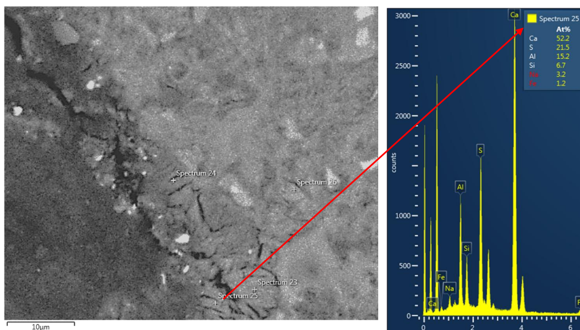
Figure 4.4: Ettringite-thaumasite products in 50%ORE sample
