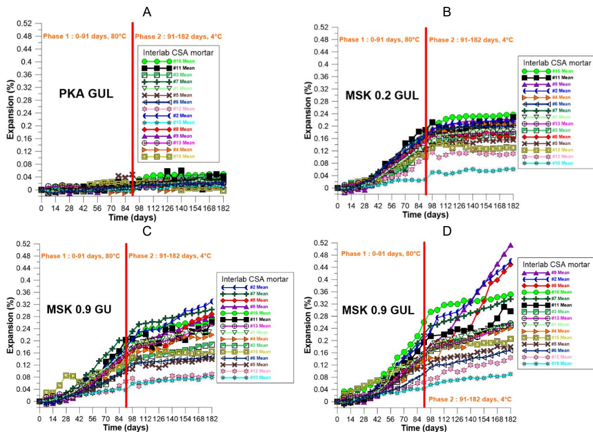
Figure 3.1: Expansion graphs of the results of the Po AMBT interlaboratory study. A: PKA with GUL cement, B: MSK 0.2% with GUL cement, C: MSK 0.9% with GU cement, D: MSK 0.9% with GUL cement.
