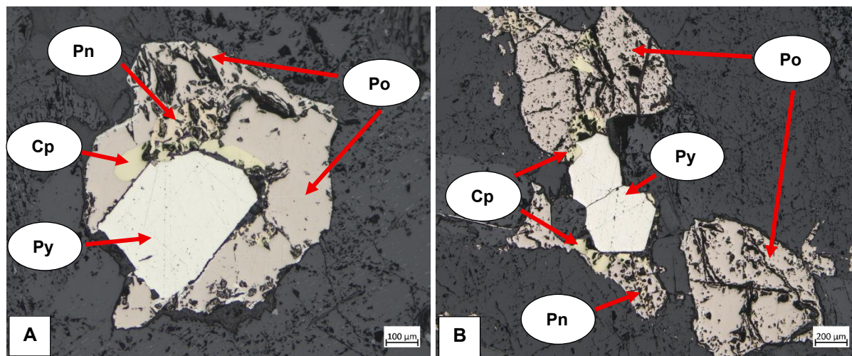
Figure 2.1: Representative reflected light images of iron-sulfide minerals. A) A single grain composed of four distinct iron-sulfide mineral phases: pyrrhotite enveloping pyrite, chalcopyrite, and pentlandite.
