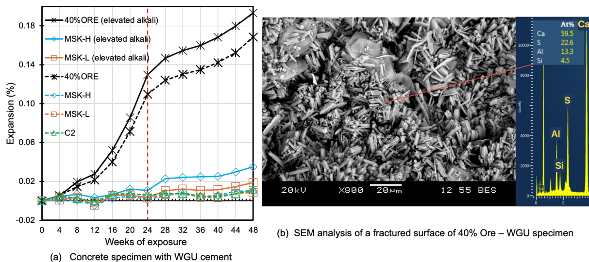
Figure 3-2: Expansion behaviour of concrete specimens containing SBA prepared with WGU (1.0% \text{Na}_2\text{O}_{\text{eq}} ). Dashed lines: saturated limewater soaking conditions. Solid lines: saturated limewater with 0.25M NaOH soaking solution. The red dashed line indicates the phase I/II transition at 24 weeks: (b) SEM image of a fractured concrete surface showing ettringite-like needles in the paste adjacent to Ore aggregates, with corresponding EDS spectrum.
