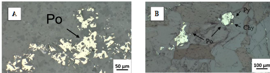
Figure 4.1: Reflected light micrographs. Po: Pyrrhotite Py: Pyrite; Chy: Chalcopyrite. [A] Epidote hornfels (C). [B] Coarse-grained garnet gneiss (M).
