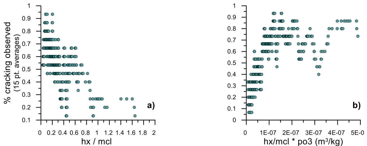
Figure 4: Likelihood of concrete deterioration as a function of a) hx/mcl and b) hx/mcl*po3. For more information see text.
