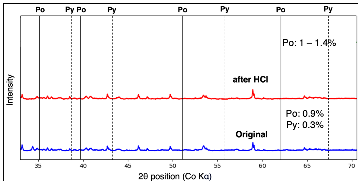
Figure 3.3: XRD diffractograms of sample from Ireland before and after the initial dissolution step. As sulfides represent only a small portion of the total mineral assemblage, their characteristic peaks are not well resolved by XRD.
