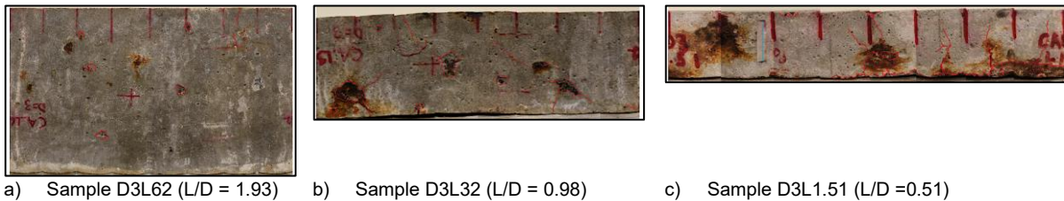
Figure 4: Surface cracking of 76 mm diameter specimens with varying L/D after 3 weeks of electrochemical exposure.
