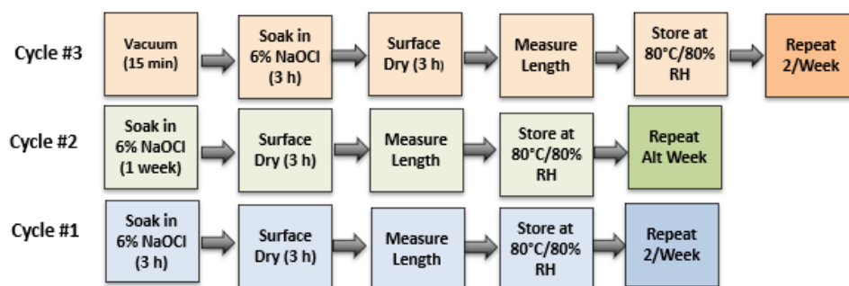
Figure 2.1. Schematic representation of accelerated oxidation–expansion testing cycles (Cycle #1: baseline after Rodrigues et al. [8]; Cycles #2–3: parametric investigations).
