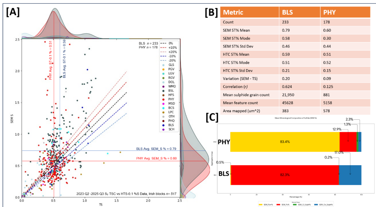
Figure 4.2: [A] ST TSC vs HTC-0.1%S Data, Irish blocks with modal distribution plots [B] key metrics for PHY and BLS groups [C] mean sulphide proportions for groups from mass data
