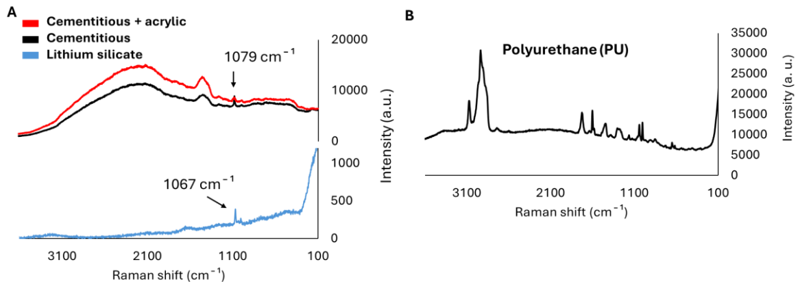
Figure 3.3: Raman spectra for concrete sealants A) cementitious types using 785 nm excitation (25mW) and B) polyurethane using 532 nm excitation (6.25 mW).
