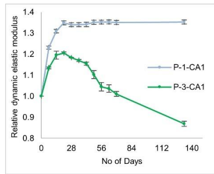
Figure 3.2: Relative E_{dyn,c} plots for P-1-CA1 and P-3-CA1 specimens during EAT
