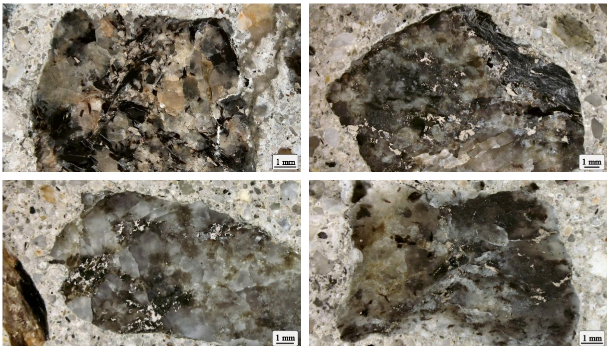
Figure 3: Representative examples of the reactive, pyrrhotite-bearing A/W coarse aggregate particles; the upper photos show gneiss particles and the lower photos show micaceous quartzite particles.
