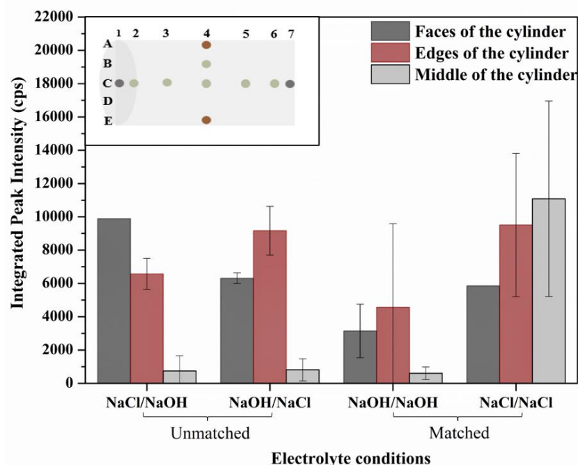
Figure 3.4: Comparison of calcite integrated peak intensities from XRD analysis across matched and unmatched electrolyte exposure configurations, highlighting variations in carbonation progression.
