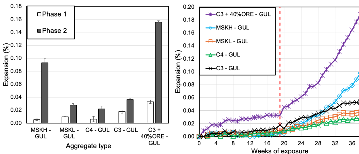
Figure 2-2: Bleach-Injection Conditioning of Concrete Micro-Prism Specimens under a Two-Phase Exposure System (19 Weeks per Phase)
