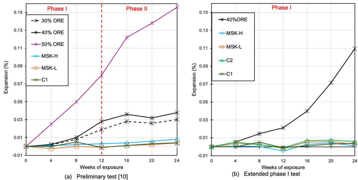
Figure 3-1: Expansion behaviour of SBA under oxygen-rich chamber exposure soaked in saturated limewater: (a) GU cement in phase I & II, each lasting 12 weeks; (b) White GU cement with 1.0% \text{Na}_2\text{O}_{\text{eq}} in phase I only lasting 24 weeks.
