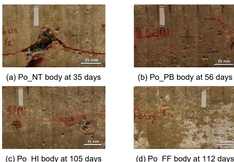
Figure 3.4: Crack mapping at the end of EAT (Group 3)
