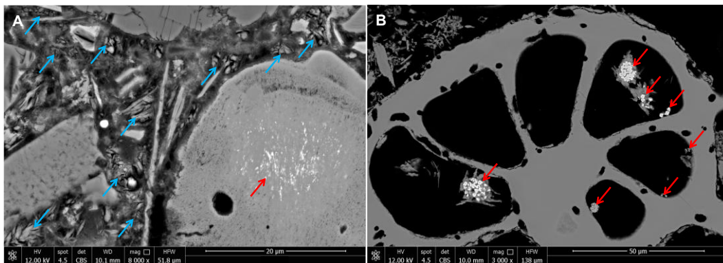
Figure 3.3: A: Partly oxidized pyrrhotite in shell particle (red arrow) and secondary ettringite (blue arrows) formed in the adjacent cement paste (HWF = 51.8 \mu\text{m} ). Outer leaf. B: Partly oxidized framboidal pyrite clusters (red arrows) in shell particle (HWF = 138 \mu\text{m} ). Inner leaf.
