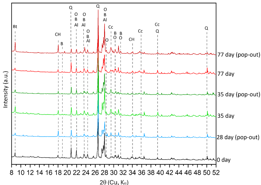
Figure 3.1: XRD pattern of P-34-CA1 samples of different oxidation and carbonation phases (Bt-biotite (9002307), CH-portlandite (9000113), Q-quartz (5000035), Al-albite (9000526), B-bytownite (9011200), O-oligoclase (9011423), Cc-calcite (45024421)).
