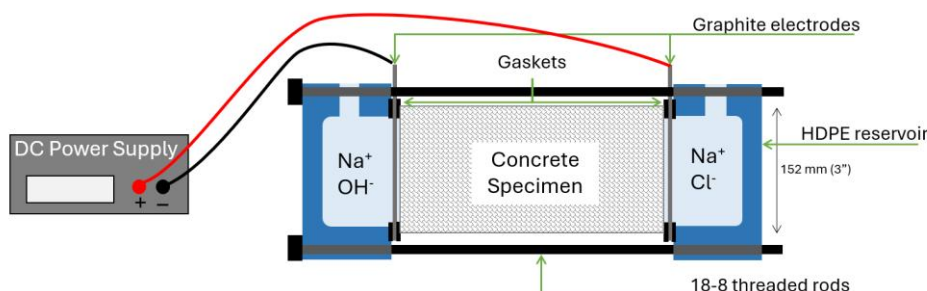
Figure 2.1. Configuration of experimental procedure (Adapted from Ojo et al. [9])
