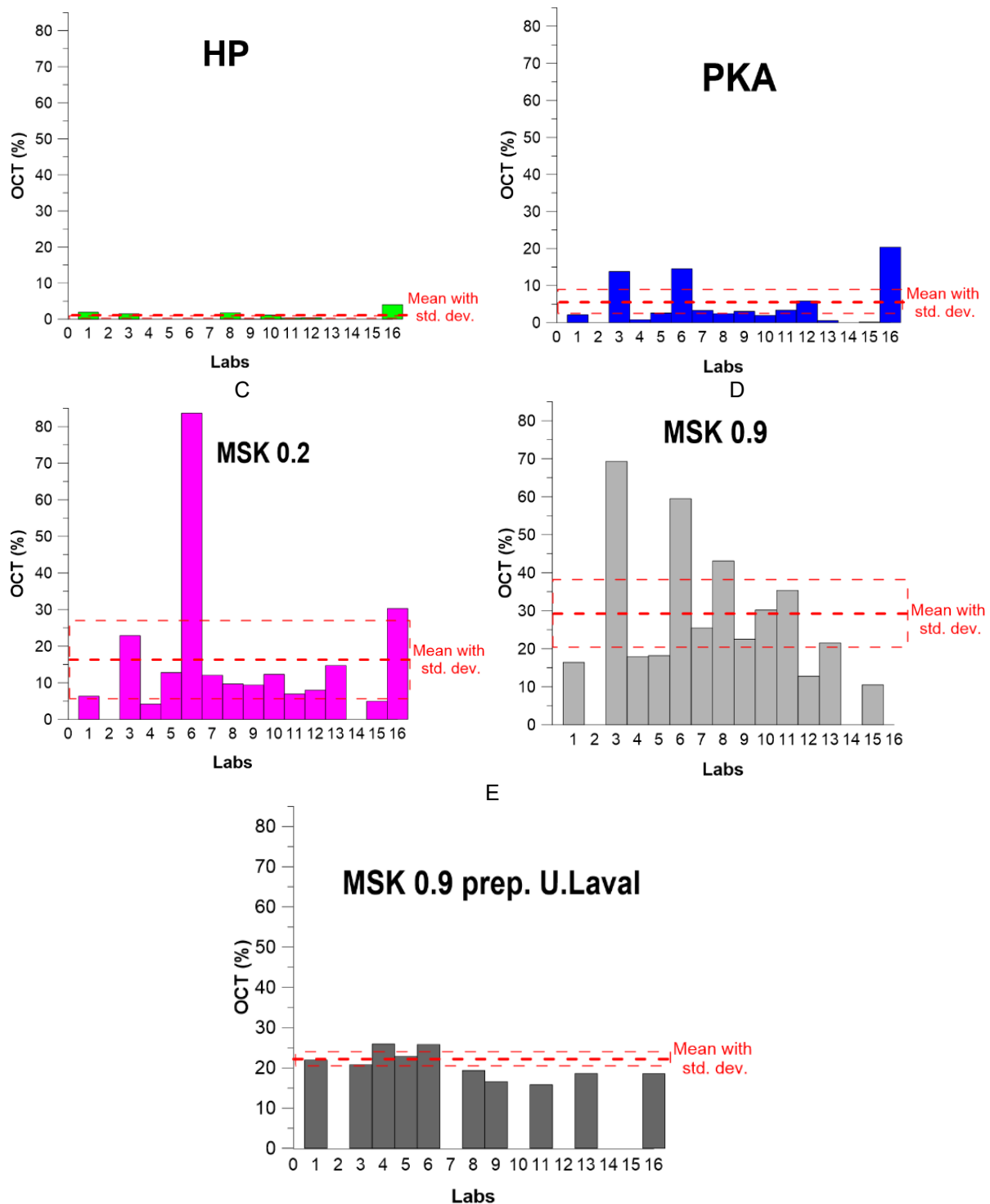
Figure 3.1: Bar charts illustrating the results (means and standard deviations) of OCT interlaboratory study (second trial). A: OCT results for non-reactive HP, B: OCT results for non-reactive PKA, C: OCT results for marginally-reactive MSK 0.2%, D: OCT results for highly-reactive MSK 0.9%, E: OCT results for MSK 0.9% prepared by U. Laval.
