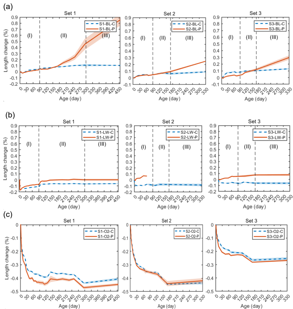
Figure 3.1: Measured length change over time for (a) Condition I: cyclic immersion in bleach solution, (b) Condition II: cyclic immersion in limewater solution, and (c) Condition III: (constant exposure to atmospheric oxygen. Phases I and II involve storage at 80°C/80% RH and 4°C/100% RH, respectively,
