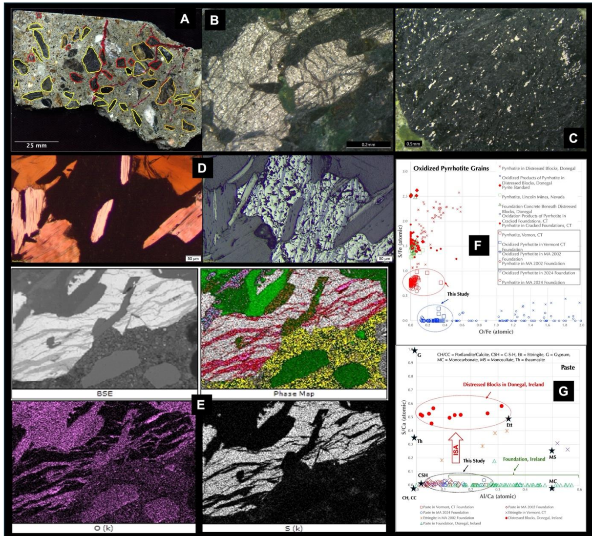
Figure 6: The Rutland, MA foundations. A: Polished cross section of a fragment where extensively and moderately pyrrhotite-bearing schist aggregates are marked by peripheral red and yellow lines, respectively, whereas non-pyrrhotite quartzite aggregates are marked in beige lines; a crack is marked in red line. B: Coarsely crystalline, subhedral to anhedral oxidized pyrrhotite grains showing characteristic striations. C: Finely disseminated forms of pyrrhotite either in random scattered grains or aligned along the weak planes of schistosity. D: Close association of pyrrhotite and biotite often one engulfed into another. E (four images): Backscatter electron image and phase map of an oxidized pyrrhotite from the elemental maps of oxygen (in pink) and sulfur (in white), omitting calcium for paste (in yellow) showing oxidized iron striations in iron sulfide matrix. F: SEM-EDS studies of iron oxide bands in oxidized pyrrhotite grains plotted in S/Fe vs. O/Fe atomic ratios from this study, other crumbled foundations from the eastern CT, and a few distressed concrete blocks and foundations from County Donegal, Ireland. G: SEM-EDS studies of paste showing the absence of elevated sulfate in the paste of dense concrete foundations from the eastern US or in some foundations in County Donegal, Ireland compared to the elevated sulfate levels (S/Ca atomic 0.4-0.6) from ISA in the distressed blocks of Ireland. Absence of elevated sulfate in the dense paste of foundations, however, does not necessarily indicate the absence of ISA when all available sulfate in the pore solutions are being used up in formation of ettringite in the confined spaces in paste to cause additional expansion and damage beyond the oxidative damage.
