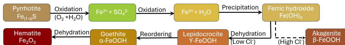
Figure 2.2. Conceptual pathway for possible Fe-bearing product formation during pyrrhotite oxidation.
