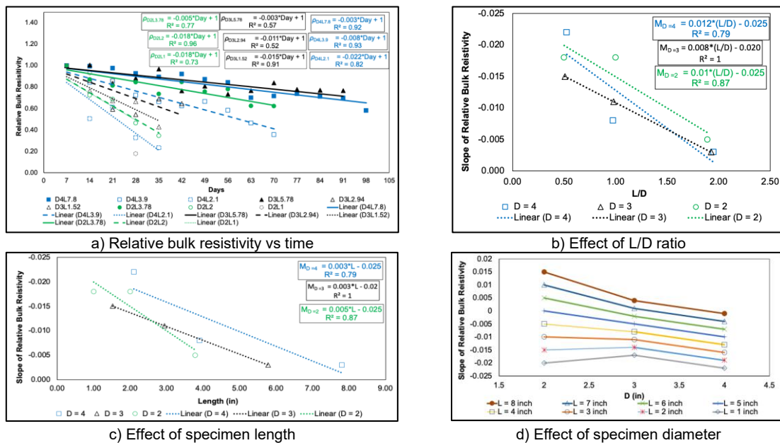
Figure 2: Influence of sample geometry on bulk electrical resistivity evolution of CA1 concrete
