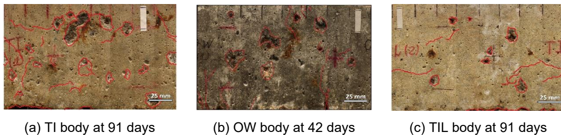
Figure 3.1: Crack mapping at the end of EAT (Group 1)
