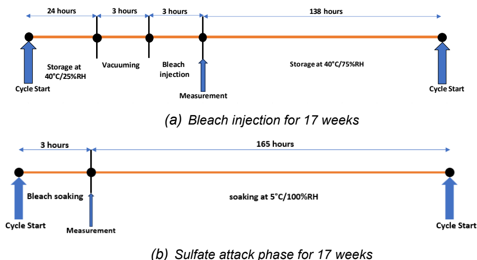
Figure 3.1: VBIT conditioning schematic details
