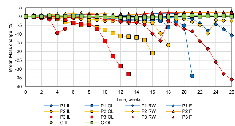
Figure 3.3 Mean mass change of each element from the three test properties and the control property over the duration of the test. Note that the mean values for each element are presented, therefore where a set of readings ends before 26 weeks this represents the failure of the last sub-sample. Where a series
