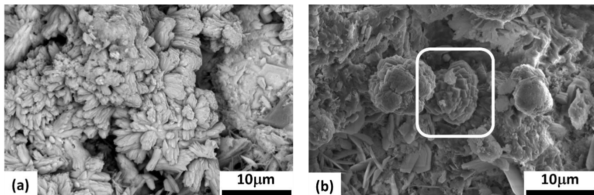
Figure 6.2: SEM of 28 day pop-out of P-34-CA1 sample showing presence of (a) scalenohedral calcite, through-the-lens BSE image, 10 kV and (b) rhombohedral calcite, ETD-SE image, 10 kV.
