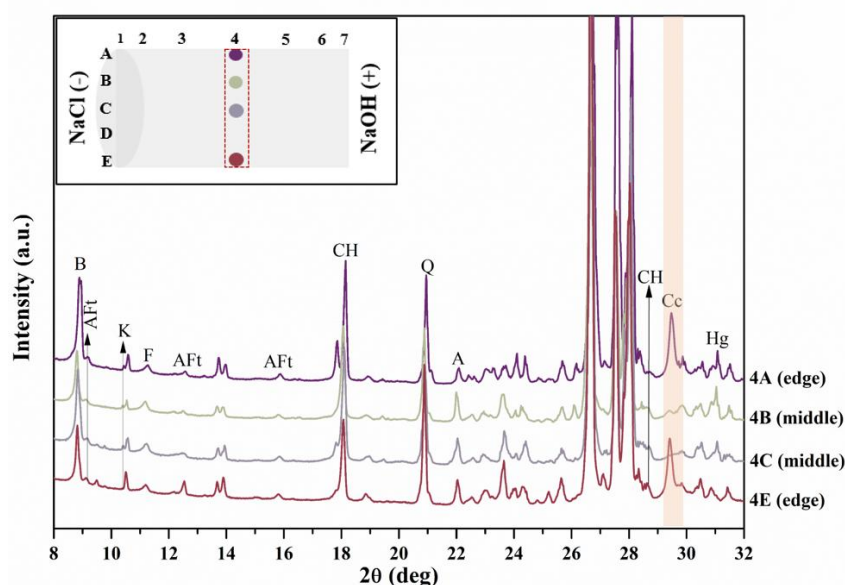
Figure 3.3: XRD profiles comparing interior and peripheral regions of specimens subjected to NaCl/NaOH exposure. Phase labels: Aft-Ettringite & Thaumasite, K-Kuzel salt, F-Friedel salt, A-Albite, and Hg-Hydrogarnet.
