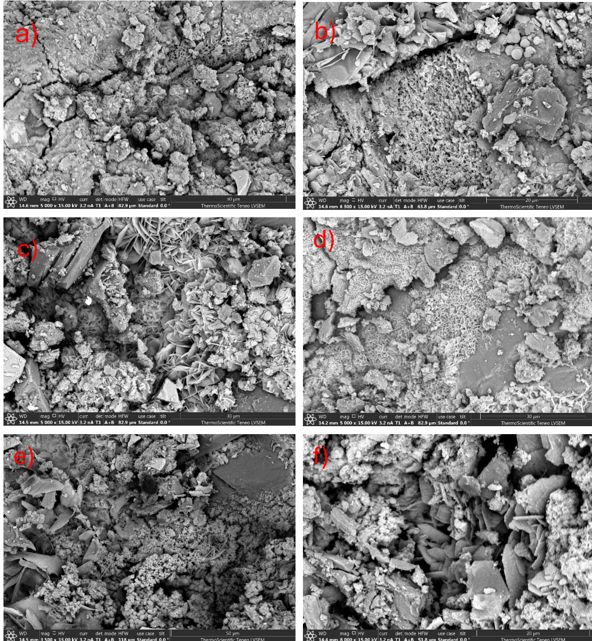
Figure 3.1. SEM micrographs showing representative Fe-rich corrosion products observed after electrochemical acceleration: (a) cotton ball-like morphology consistent with ferrihydrite-like products; (b) Fe-rich corrosion front; (c) transitional FeOOH-like morphology; (d) plate-like morphology consistent with lepidocrocite-like products; (e) acicular morphology consistent with goethite-like products; and (f) oxide-like Fe-rich product morphology.
