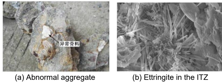
Figure 2.2: Abnormal aggregate from building 1 and ettringite in ITZ [2]
