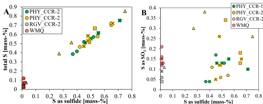
Figure 3.1: Total sulfur (S) as a function of sulfur (S) as sulfide (A) and sulfur (S) as \text{SO}_3 as a function of sulfur (S) as sulfide (B). CCR-1: data from [2], CCR-2: data from [3]. Symbols in (B): triangle = foundation concrete, square = RB, circle = OL, cross = IL.
