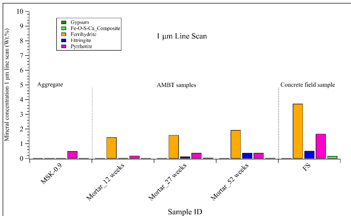
Figure 3: Concentration of pyrrhotite and secondary oxidation minerals present in the fresh aggregate (MSK-0.9), the mortar bar samples, and the concrete field sample (FS), measured by automated mineralogy using 1 µm line scanning mode.
