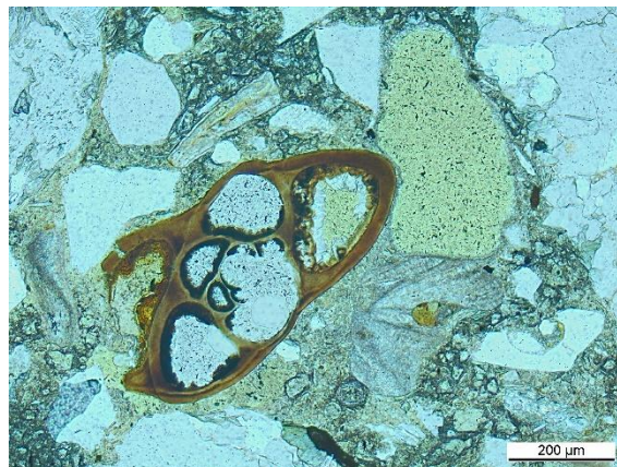
Figure 3.2: Stained shell particle with linings of opaque particles in its interior from an RB sample using polarized light.
