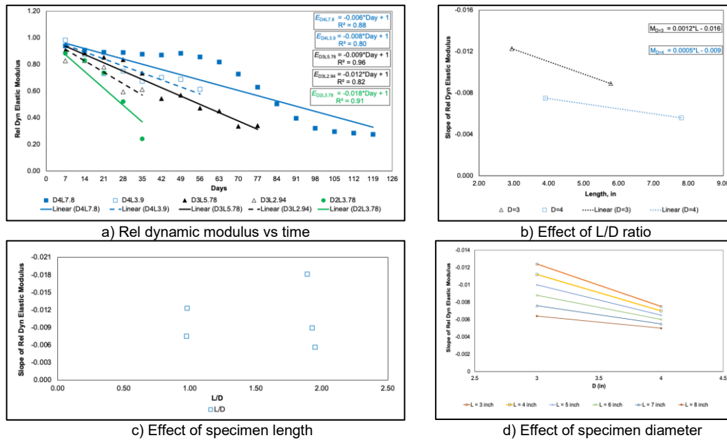
Figure 3: Effect of specimen geometry on dynamic elastic modulus degradation of CA1 concrete
