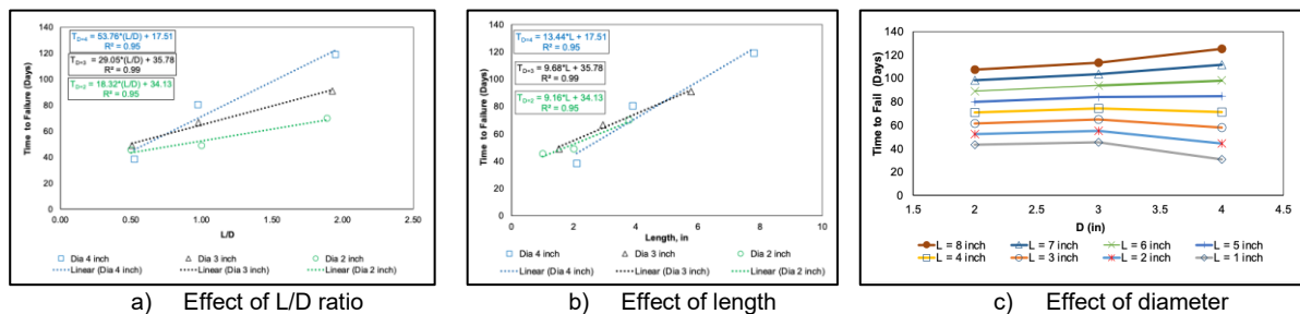
Figure 5: Effect of specimen geometry on time to failure of CA1 concrete
