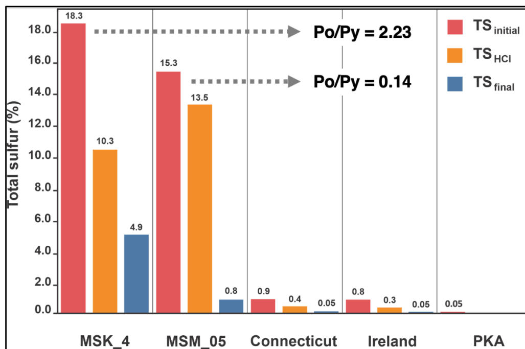
Figure 3.1: Total sulfur (TS%) results for samples with different sulfur contents subjected to the dissolution protocol. The sulfur-rich samples MSK_4 and MSM_05 were analyzed by XRD to track mineralogical evolution during the dissolution stages and their respective Po/Py original ratios were independently verified by SEM-QEMSCAN.
