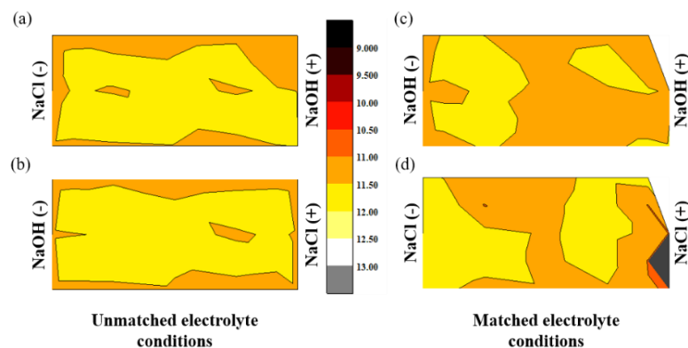
Figure 3.1: Spatial variation of pH measurements in concrete specimens after EAT under four electrolyte configurations: (a) NaCl/NaOH, (b) NaOH/NaCl, (c) NaOH/NaOH, and (d) NaCl/NaCl.
