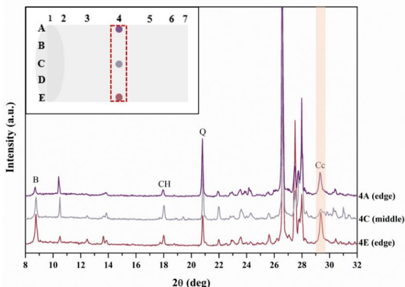
Figure 3.2. XRD pattern of non-accelerated (NA) concrete, showing calcite enrichment near surfaces and limited presence within the matrix. Phase labels: B-Biotite, CH-Portlandite, Q-Quartz, Cc-Calcite
