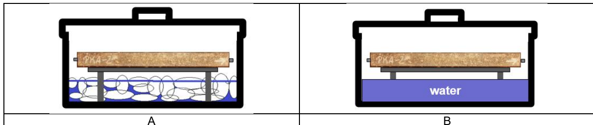
Figure 2.1: Po AMBT phases I and II testing regime schematics. A: Phase I testing regime - mortar bars are supported by ABS pipe sections and plastic grid over supersaturated NaCl solution to maintain 75% R.H. at 80^\circ\text{C} . B: Phase II testing regime – mortar bars are supported by the same setup over tap water to maintain 100% R.H. at 4^\circ\text{C} .
