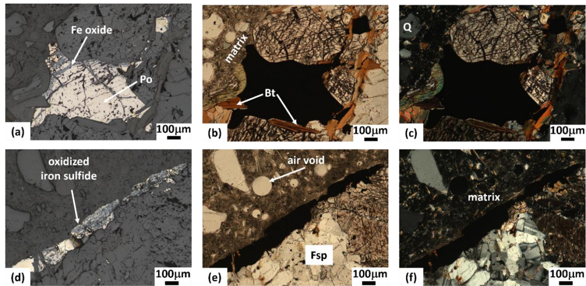
Figure 3.3: Thin section petrographic images of untested P-34-CA1 sample with particular focus on oxidized iron sulfides and its surroundings; (a) and (d) reflected light images, (b) and (e) plane polarized transmitted light images, (c) and (f) cross polarized transmitted light images. Key: Po (Pyrrhotite), Bt (Biotite), Fsp (Feldspar), Q (Quartz)
