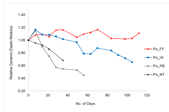
Figure 3.5: Relative E_{dyn,c} over number of days (Group 3)
