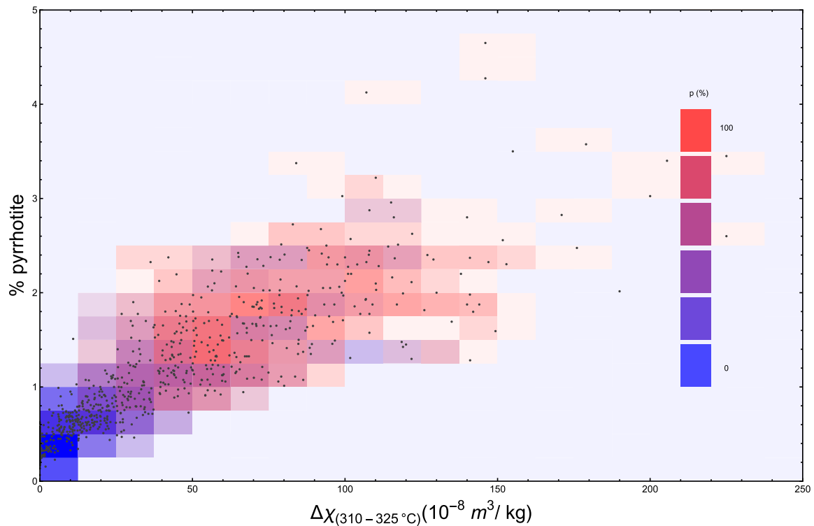
Figure 3: Likelihood of concrete deterioration. Total % pyrrhotite estimated from sulphur concentrations, change in susceptibility as shown in Figure 1b. Hue indicates likelihood of failure (red = 100%, blue = 0%), lightness of hue indicates number of structures that were used to calculate failure rate.
