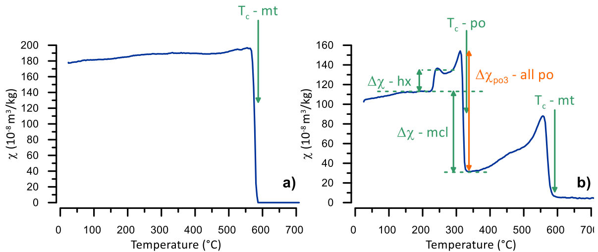
Figure. 1: Examples of thermomagnetic curves. a) sample containing magnetite b) sample containing both pyrrhotite and magnetite. For further information see text.
