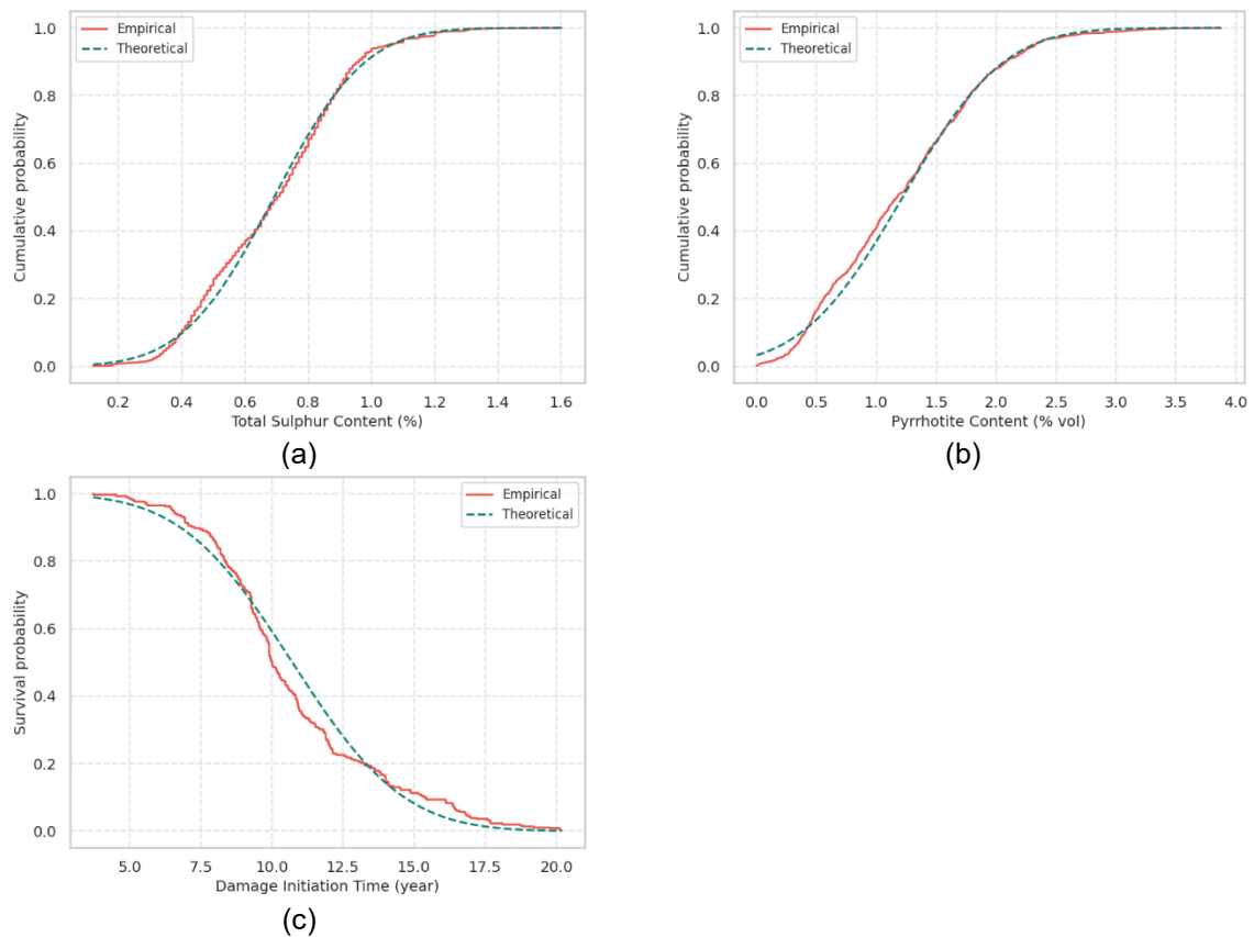
Figure 5.2: Theoretical and empirical cumulative probabilities of damaged concrete elements for (a) total sulphur content; (b) pyrrhotite content and (c) damage initiation time
