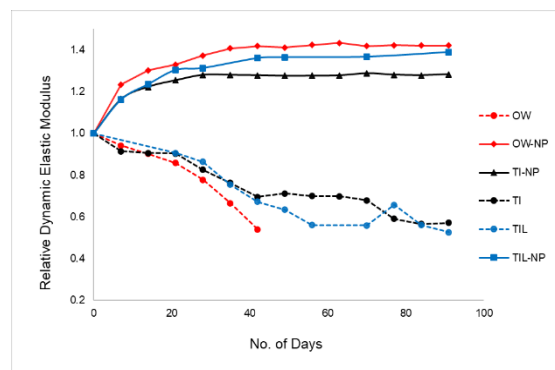
Figure 3.2: Relative E_{dyn,c} over number of days (Group 1)
