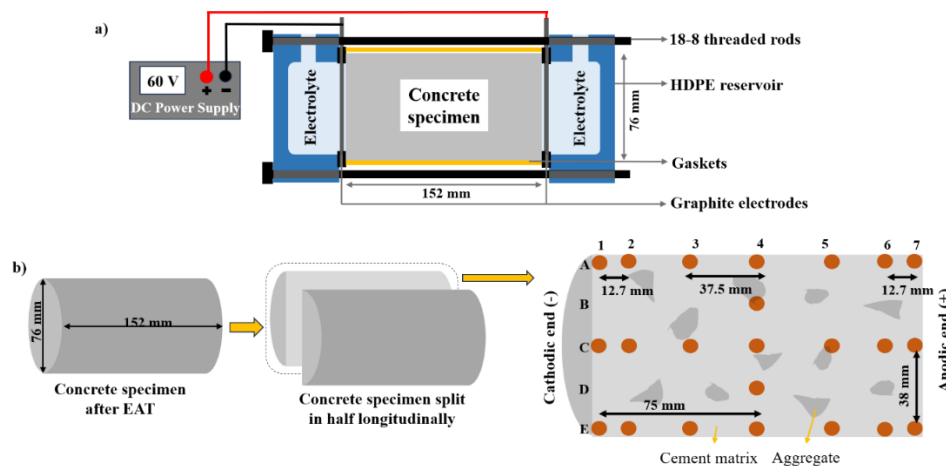
Figure 2.1: (a) Schematic representation of the EAT setup (b) Location and spacing of the spots considered for compositional analysis.
