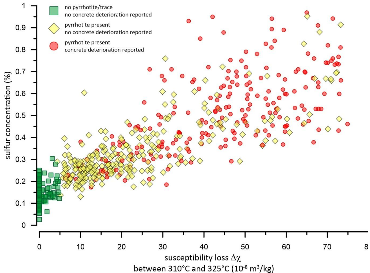
Figure 2: Total sulphur concentration (in % S) as a function of pyrrhotite abundance as determined by thermomagnetic analyses for over 1000 homes in Connecticut and Massachusetts. The status of the investigated structure is also indicated.
