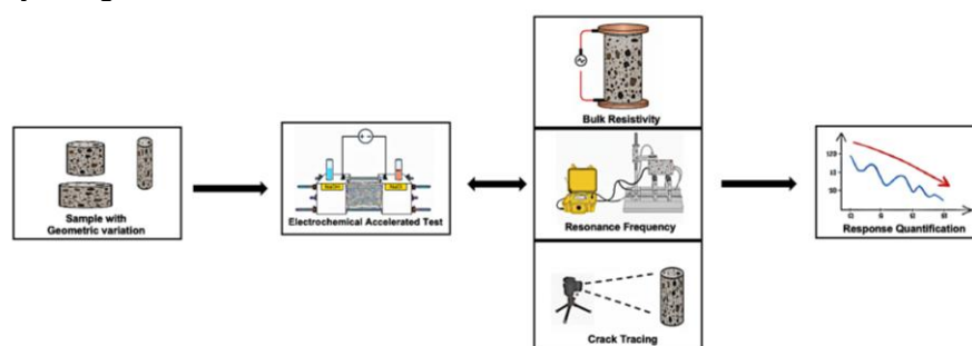
Figure 1: Experimental workflow for accelerated deterioration testing.
