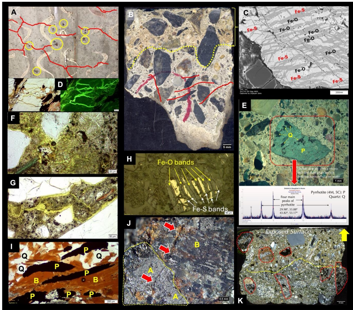
Figure 5: The Vernon, CT home. A: Extensive cracking (red lines) and popouts of oxidized pyrrhotite grains (circled) in the foundation wall. B: A polished concrete fragment showing beige discoloration at the exposed surface end of wall from atmospheric carbonation (depth of carbonation is 30-mm, which is marked by yellow dotted line as the carbonation front); visible cracks are marked with red lines. C: Backscatter electron image of a polished section of extensively cracked oxidized pyrrhotite grain showing alternate darker gray Fe-O and brighter Fe-S bands. D: Micrograph of thin section of an extensively cracked pyrrhotite-bearing coarse aggregate where cracks are highlighted by fluorescent dye in the corresponding image taken in the UV light. E: A sand-size 'chunk' of pyrrhotite with minor quartz inclusions, which has shown a spectacular four-peak diffraction pattern of 4M pyrrhotite. F: Micrograph of thin section showing extensive contamination and mixing of fibrous, acicular ettringite in cement paste, i.e., beyond the usual filling of voids and cracks by secondary ettringite, such ettringite-infested paste is the telltale evidence of ISA in paste. Ettringite-related ISA occurs only in the interior non-carbonated concrete since ettringite is unstable in the carbonated surface region of foundation, G: Cracks extending from unsound aggregates to interstitial paste, which are often filled with ettringite. H: Micrograph of polished section of oxidized pyrrhotite in the reflected-light mode of a petrographic microscope showing alternate Fe-O and Fe-S bands. I: Thin section micrograph showing close association of elongated pyrrhotite grains with biotite flakes in aggregate, where such juxtaposition pyrrhotite within biotite has facilitated easy access of oxygen and moisture for oxidation through the biotite flakes. J: A pyrrhotite 'chunk' in a gneiss coarse aggregate showing one half of less oxidized (marked as 'A') and other half of extensively oxidized pyrrhotite, latter with parallel Fe-S bands (marked as 'B'), and a crack traversing the grain (red arrows) developed from oxidation. K: Large-area (50 × 75 mm) thin section scanned on a flatbed transparent scanner showing pyrrhotite-bearing aggregates (marked by red dotted lines) where thin section was sandwiched between two perpendicular polarizing filters to recreate cross-polarized light view of a petrographic microscope.
