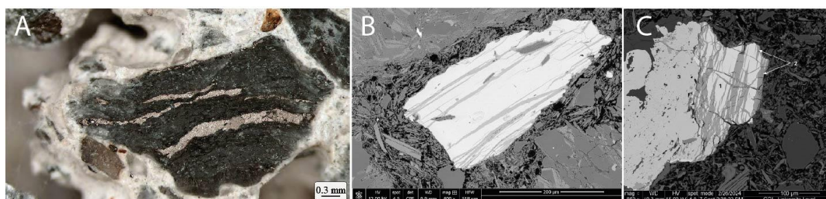
Figure 1. A shows pyrrhotite bands clearly identified in concrete aggregates (CRT). B (Empa) C (Laval) SEM images of pyrrhotite with oxidized regions.
