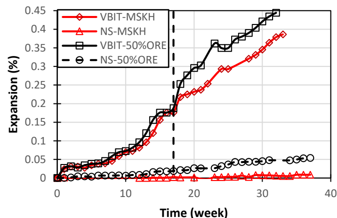
Figure 4.2: Comparison of VBIT with Normal Bleach Soaking conditionings
