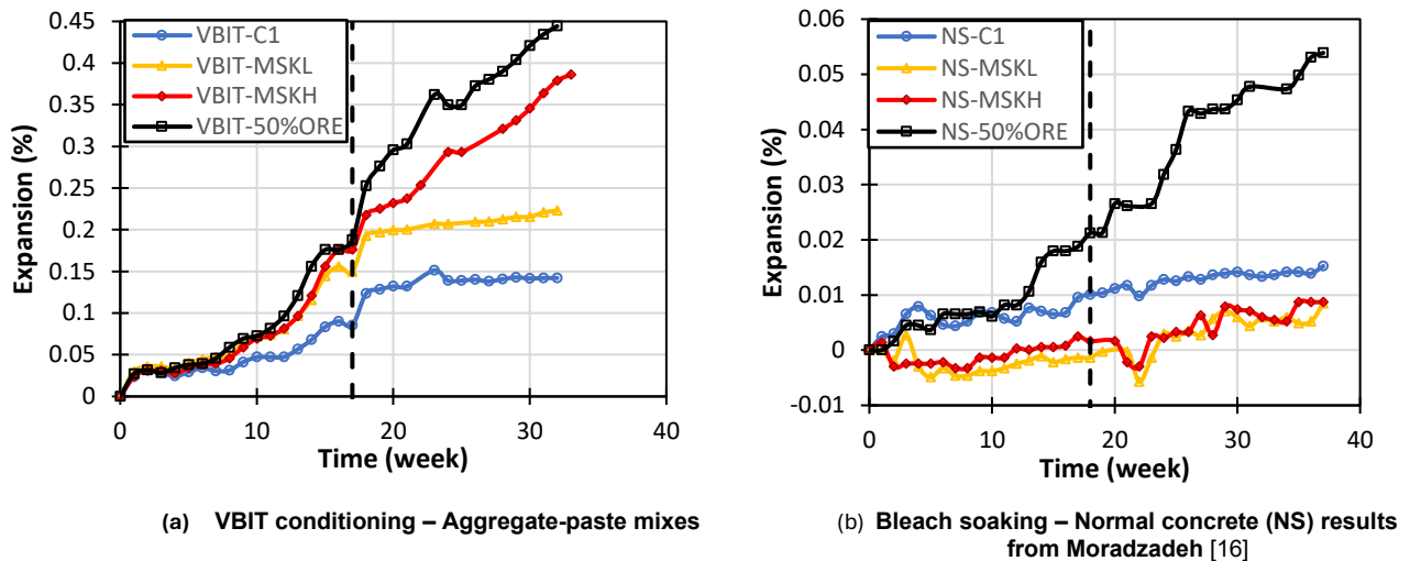
Figure 4.1: VBIT and Normal Bleach Soaking expansion results – Different scale of the Y-axes
