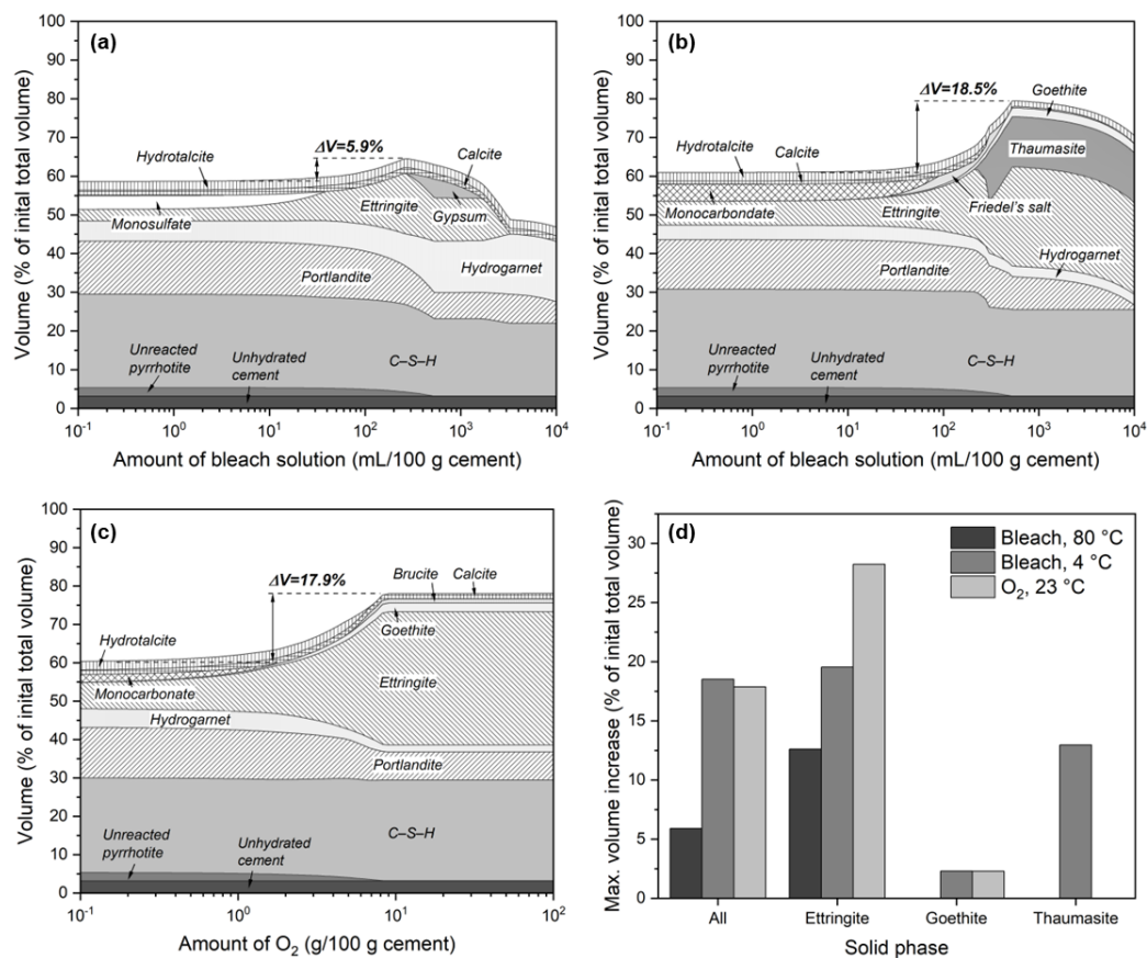
Figure 3.2: Predicted phase assemblages upon exposure to (a) bleach at 80°C, (b) bleach at 4°C, and (c) atmospheric oxygen at 23°C. A comparison of the phase assemblages is summarized in panel (d).
