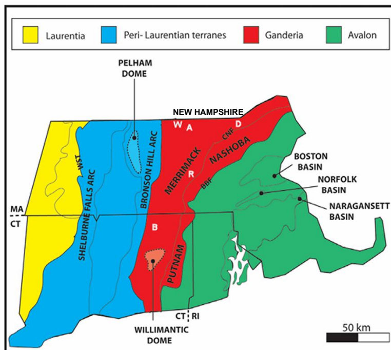
Figure 1: Simplified tectonic map of Southern New England [8]. Major structural features are marked: BBF=Bloody Bluff Fault; CNF=Clinton-Newbury fault zone, WST=Whitcomb Summit thrust zone. Referenced locations in the paper are marked: B=Becker Quarry, R=Rutland, W=Winchendon, A=Ashburnham, D=Dracut. All of the reactive aggregates are located in the Merrimack Terrane.
