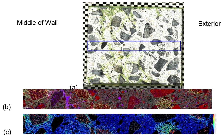
Figure 4.3: (a) The imaged subsection of the 709-F1 exterior slice; the middle of the wall is on the left and the exterior wall edge is on the right; this is consistent in subsequent images (field of view: 139 mm x 120 mm). (b) A \mu XRF chemical map of the subsection (Ca – green, Si – brown, S – yellow, Cl – purple; field of view: 128 mm x 13 mm). (c) The heat map of sulfur concentration from the \mu XRF; red is high and black is low (field of view: 128 mm x 13 mm)
