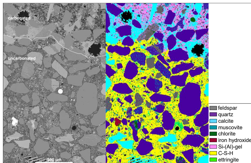
Figure 3.5: BSE-image (A) of the carbonation front (above dashed line) and phases present in the carbonated and uncarbonated cement paste (B). Outer leaf.
