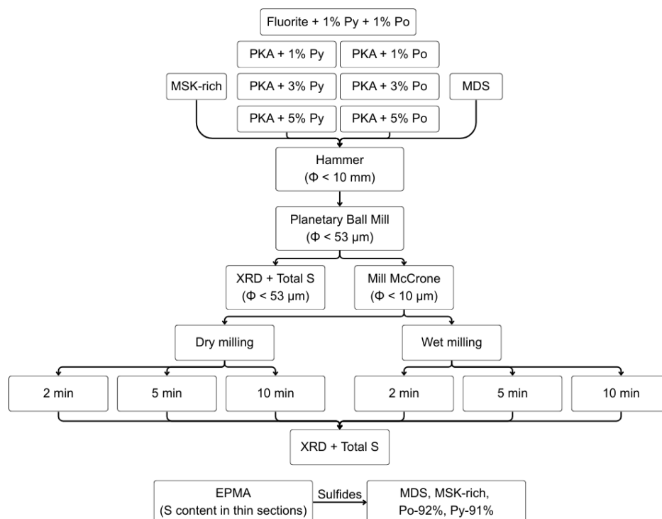
Figure 2.1. Flowchart of sample preparation and analysis of MSK-rich, MDS, PKA, and Fluorite. PKA and Fluorite were mixed with different contents of Pyh and Py. Percentages are in weight %.
