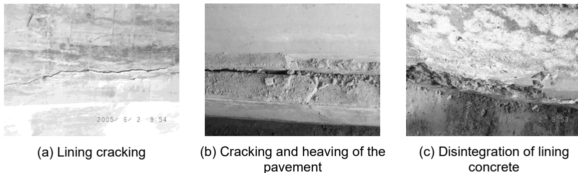
Figure 3.1: Typical deterioration characteristics of Shiziya Tunnel [3]
