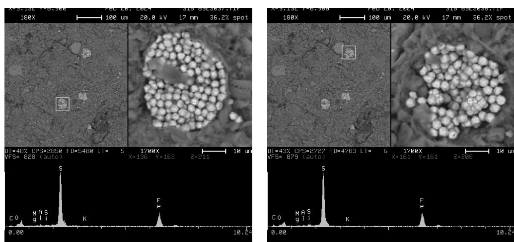
Figure 2.2: Backscattered electron (BSE) images with EDS spectra showing framboidal pyrite composed of packed, rounded microcrystals.
