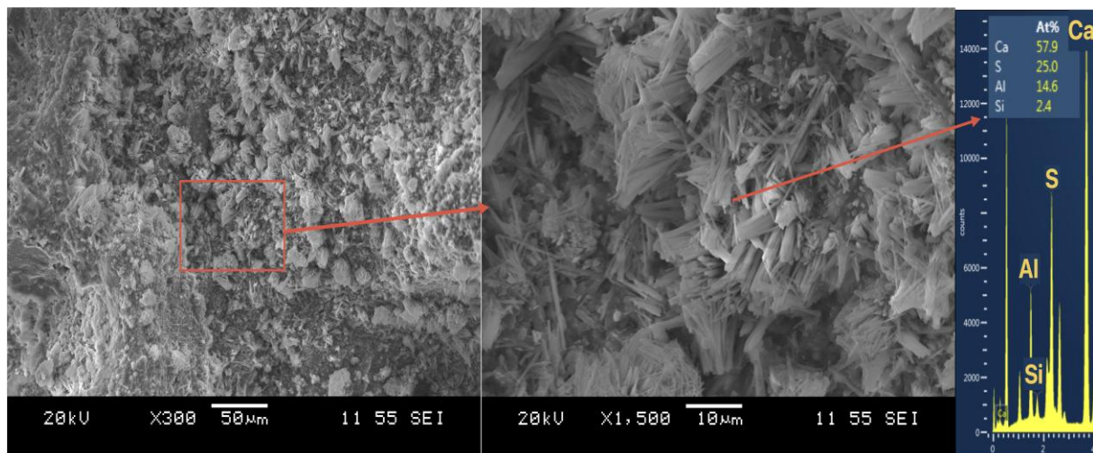
Figure 2-3: SEM-EDS of a fractured concrete surface showing ettringite-like needles in the paste adjacent to MSKH aggregates.
