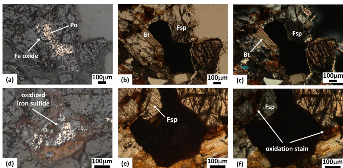
Figure 3.4: Thin section petrographic images of 77 day tested P-34-CA1 sample with particular focus on oxidized iron sulfides with and without adjacent biotite; (a) and (d) reflected light images, (b) and (e) plane polarized transmitted light images, (c) and (f) cross polarized transmitted light images. Key: Po (Pyrrhotite), Bt (Biotite), Fsp (Feldspar)
