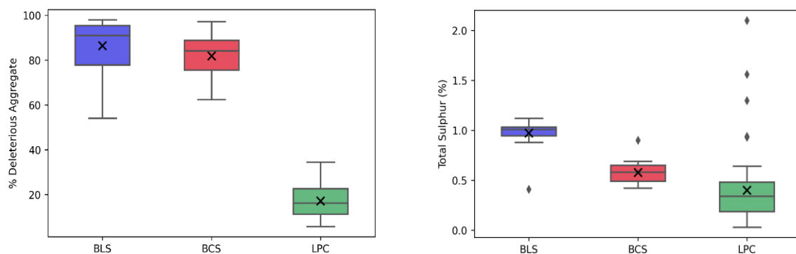
Figure 2.2: Comparative charts showing the difference in deleterious aggregate proportions (left) and total sulphur content – EN 1744, Clause 11.2 HTC (right) between the two main deleterious “mudrock” aggregates and the claystone. Due to the small sample size for LPC ( n=23 ), similar numbers of tested samples were selected for BLS and BCS ( n=21 ). TS values have a 0.1% “correction” subtracted as an assumption of the cement contribution as per I.S. 465.
