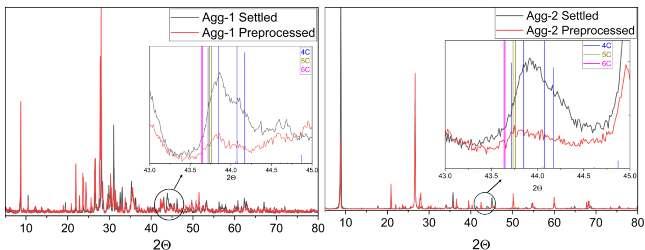
Figure 4: XRD scans of the samples before and after gravity-based separation using LMT.
