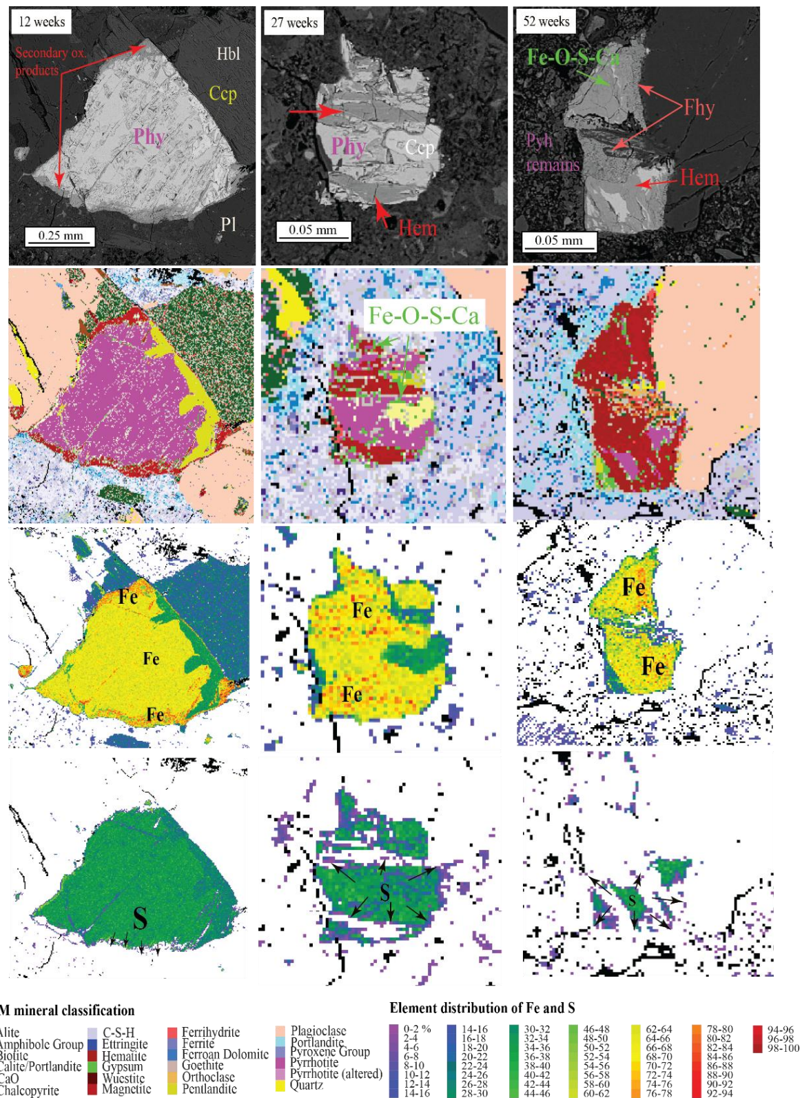
Figure 2: Oxidation progression of pyrrhotite studied in the accelerated mortar bar samples from 12 to 52 weeks. The AM mapping of the AMBT samples was obtained using a 2 µm step size. Phy remains = Pyrrhotite residues after oxidation and alteration to iron oxides and (oxi) hydroxides; Fhy = Ferrihydrite; Ccp = Chalcophyrite; Hbl= Hornblende; Pl = Plagioclase; Hem = Hematite; Fe-O-S-Ca = Composite phase.
