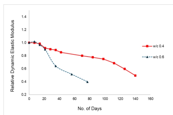
Figure 3.3: Relative E_{dyn,c} over number of days (Group 2)
