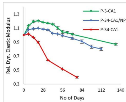
Figure 3.4: Relative E_{dyn,c} plots for P-34-CA1 and P-34-CA1/NP specimens (P-3-CA1 included)
