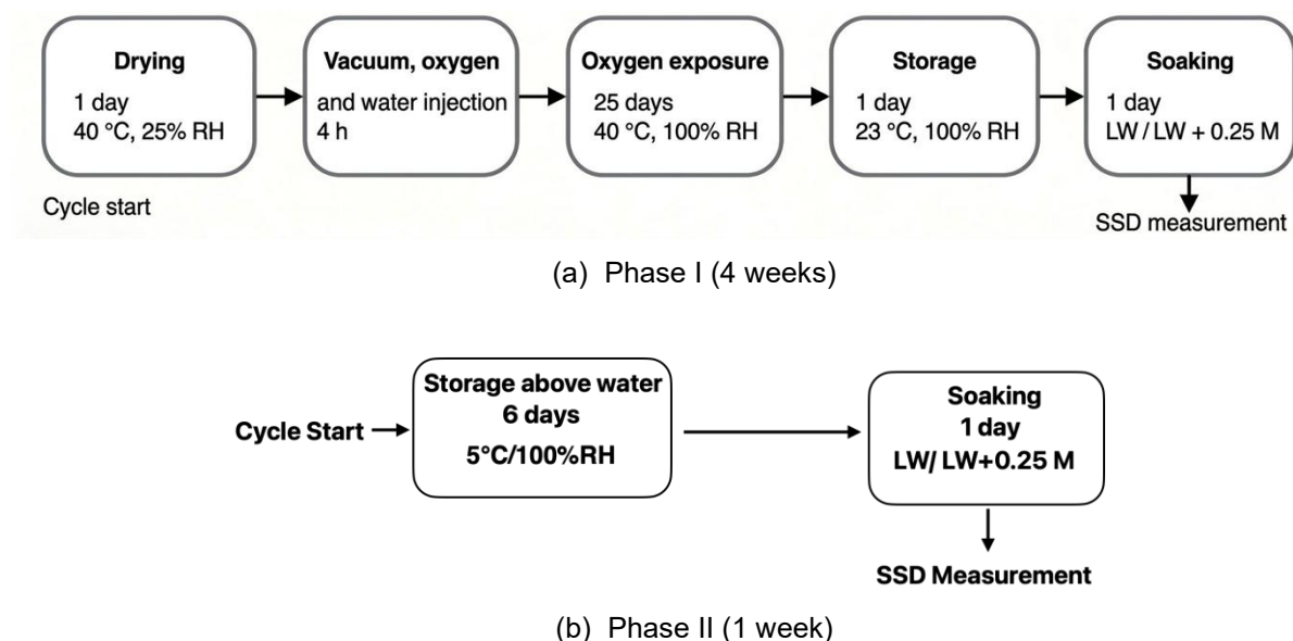
Figure 2-1: Oxygen-rich test cycles: (a) 28 days per cycle for oxidation phase; (b) sulphate attack phase (7 days per cycle).
