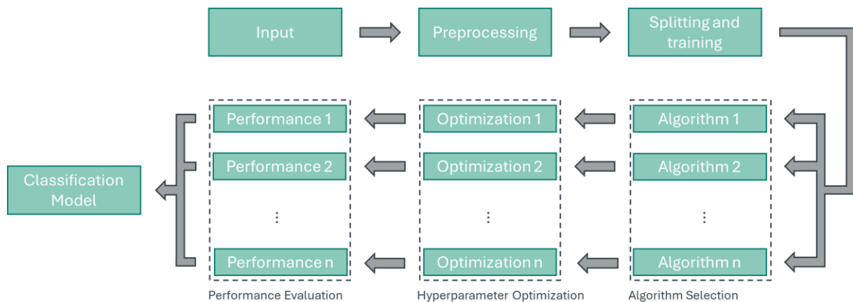
Figure 3.1: Methodological process
