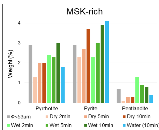
Figure 3.1. Variation in sulfide content in MSK-rich aggregate according to the sample preparation method. Results determined by Rietveld refinement (XRD).
