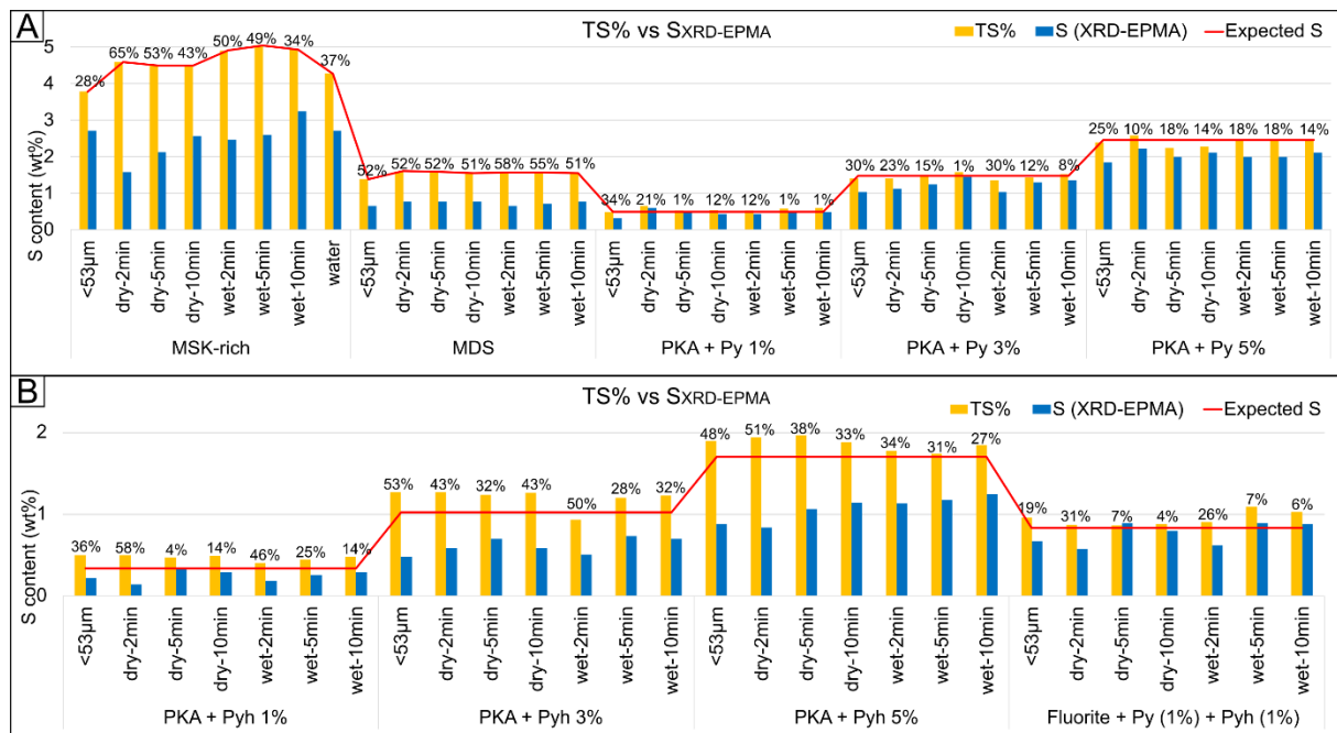
Figure 3.4. Variation between the measured sulfur from TS% vs mineralogy-derived sulfur ( S_{\text{XRD-EPMA}} ). Percentage values above the bars indicate the relative error between the two techniques.
