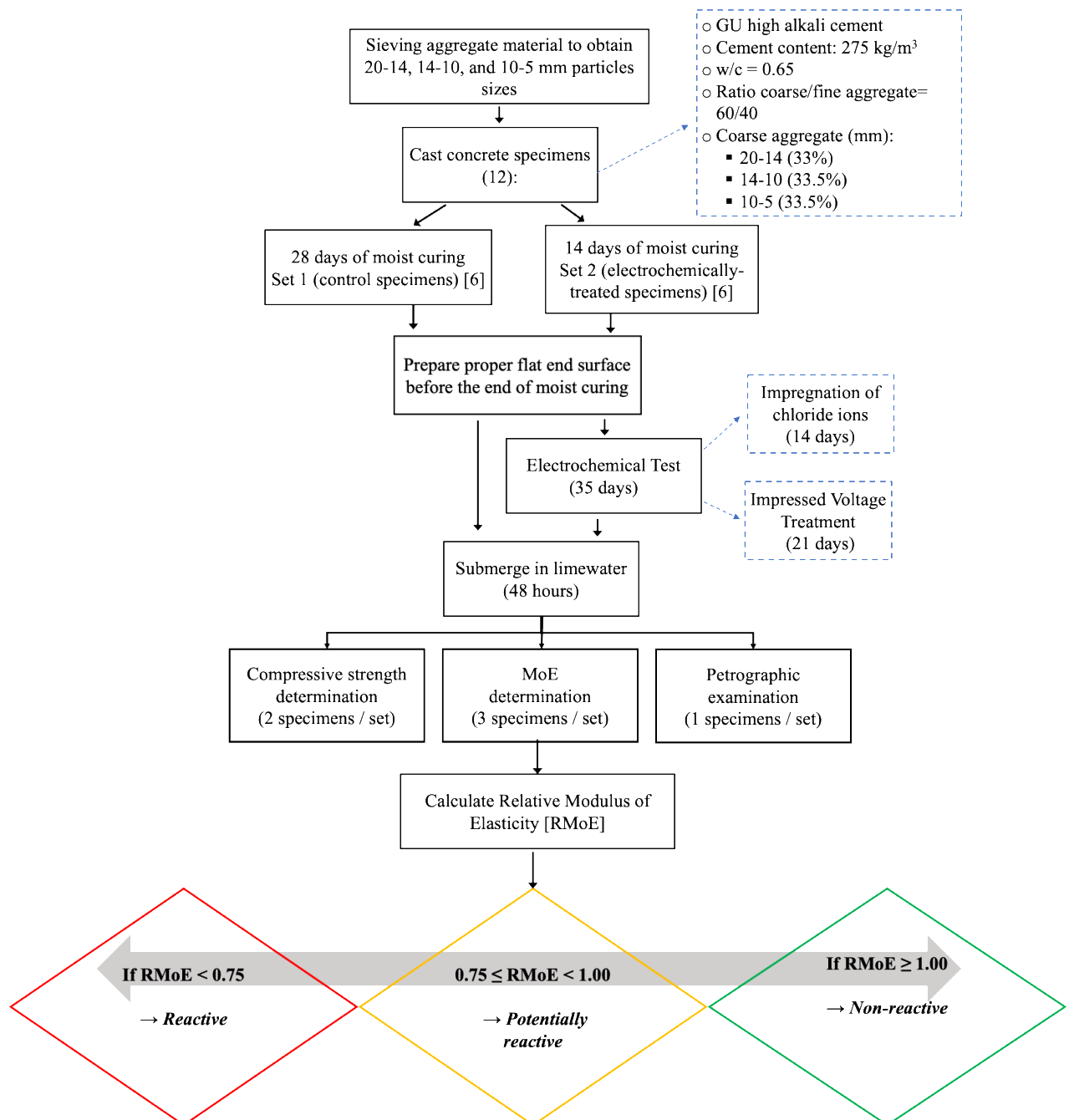
Figure 3.1: Electrochemical testing scheme proposed by Castillo Araiza et al. [5].
