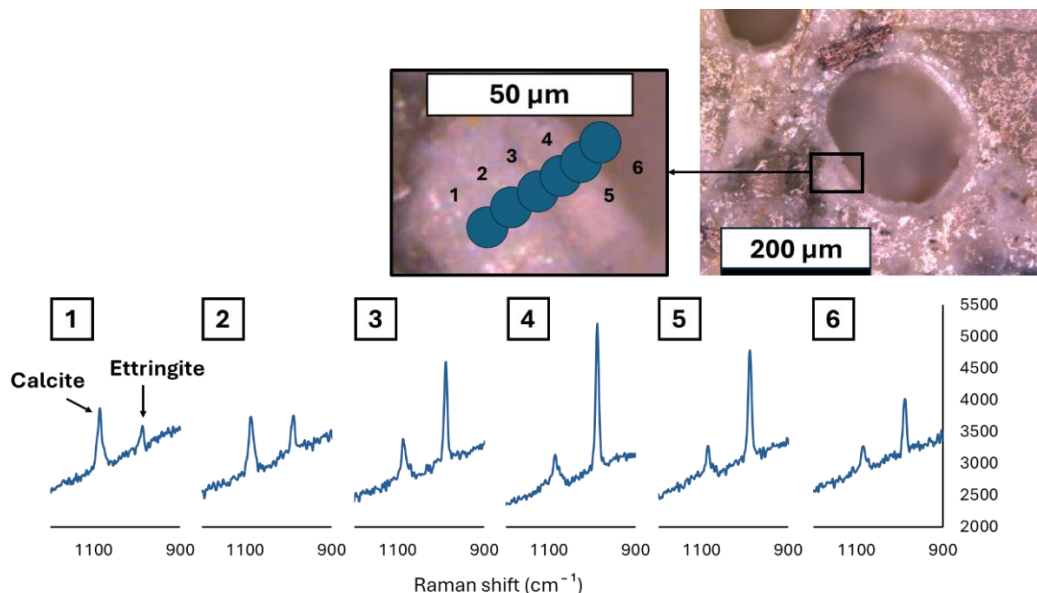
Figure 3.2: Raman spectra for concrete air void with ettringite formation using 785 nm excitation (10 mW) with 10x objective.
