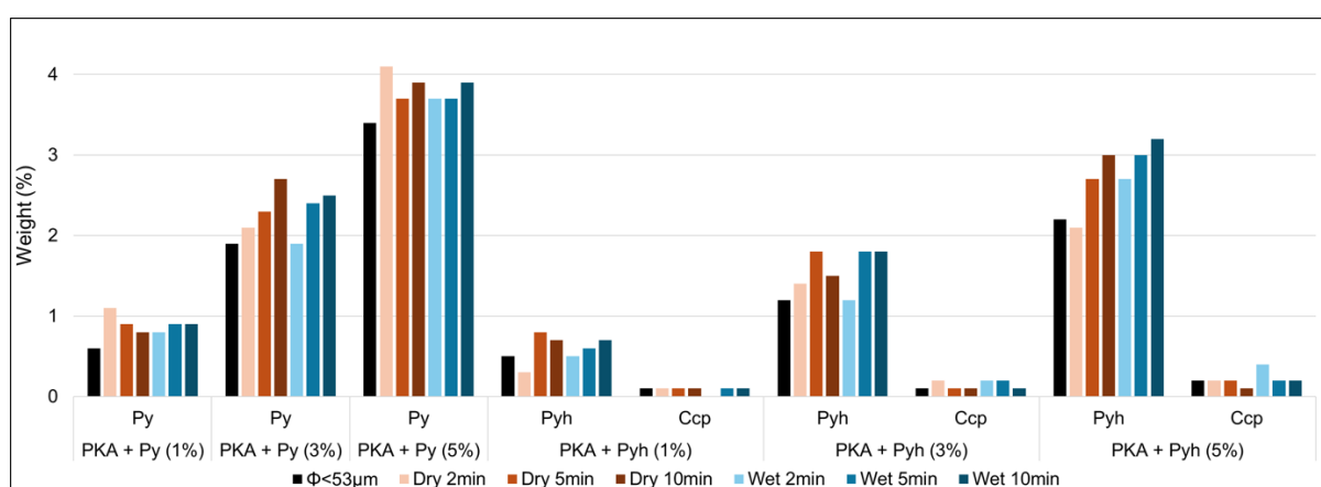
Figure 3.3. Sulfide variation according to sample preparation for all sulfide mixtures with PKA.
