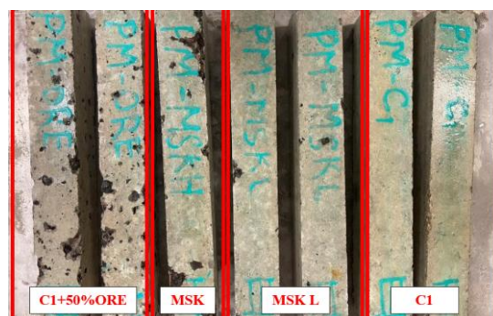
Figure 4.3: The surface of the aggregate-paste mix samples at the end of conditioning
