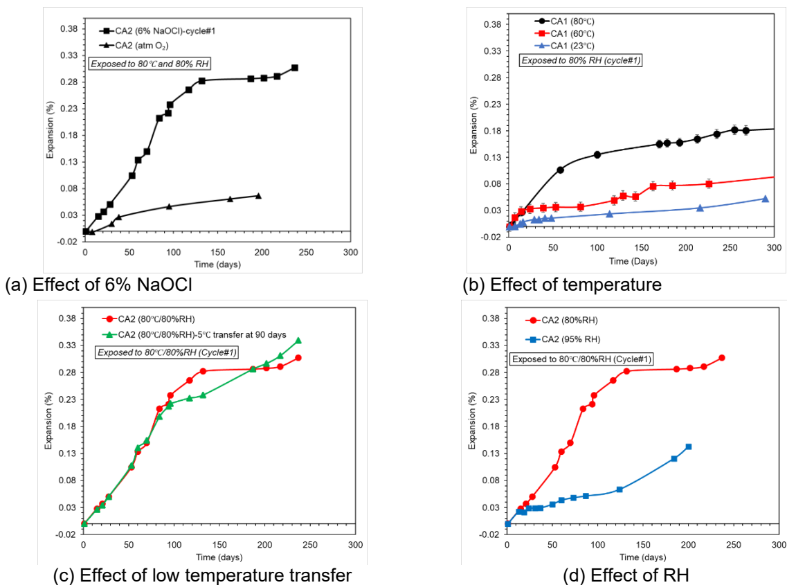
Figure 3.1. Effect of environmental exposures on the expansion of sulfide-bearing aggregate.
