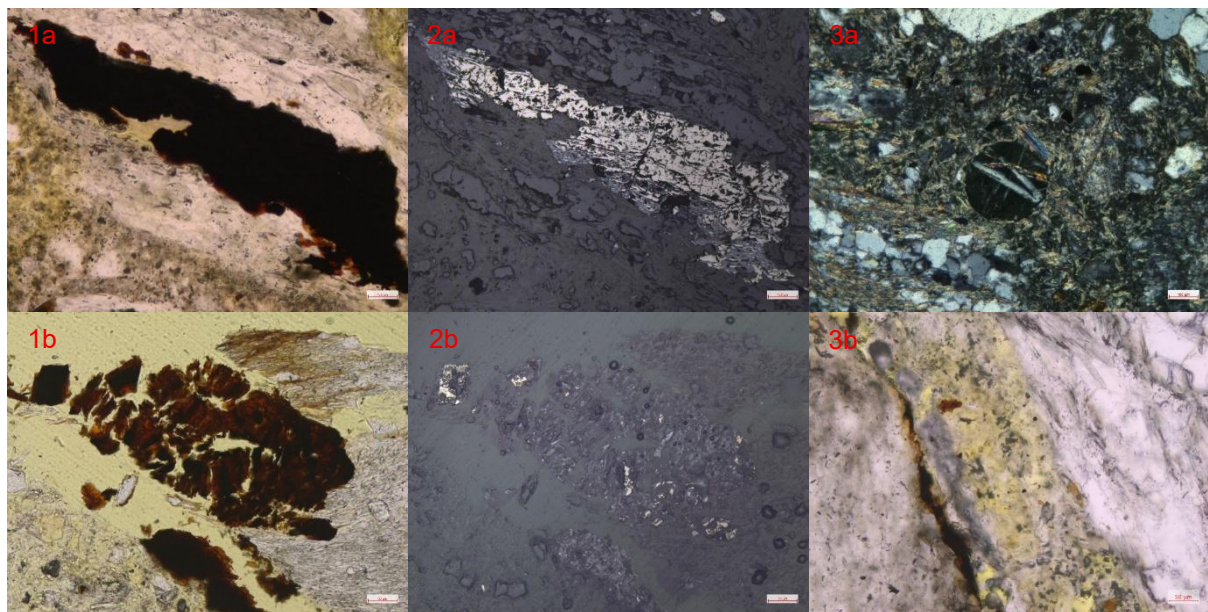
Figure 3.5 Photomicrograph examples of the test properties before (a) and after (b) the ACT showing the oxidation of the pyrrhotite in both plane polarised light (1a and 1b) and reflected light (2a and 2b), and the internal sulfate attack products (3a, gypsum XPL and 3b, ettringite PPL).
