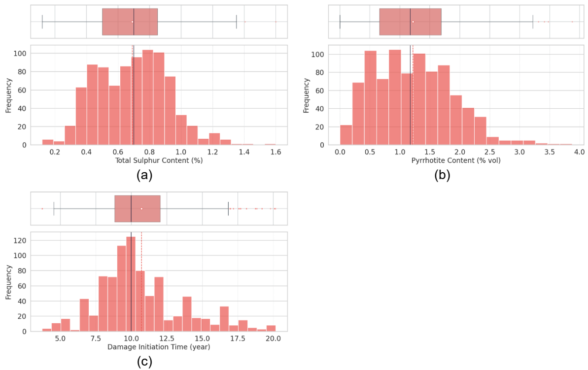
Figure 5.1: Distribution of damaged concrete in function of (a) total sulphur content, (b) pyrrhotite content and (c) damage initiation time
