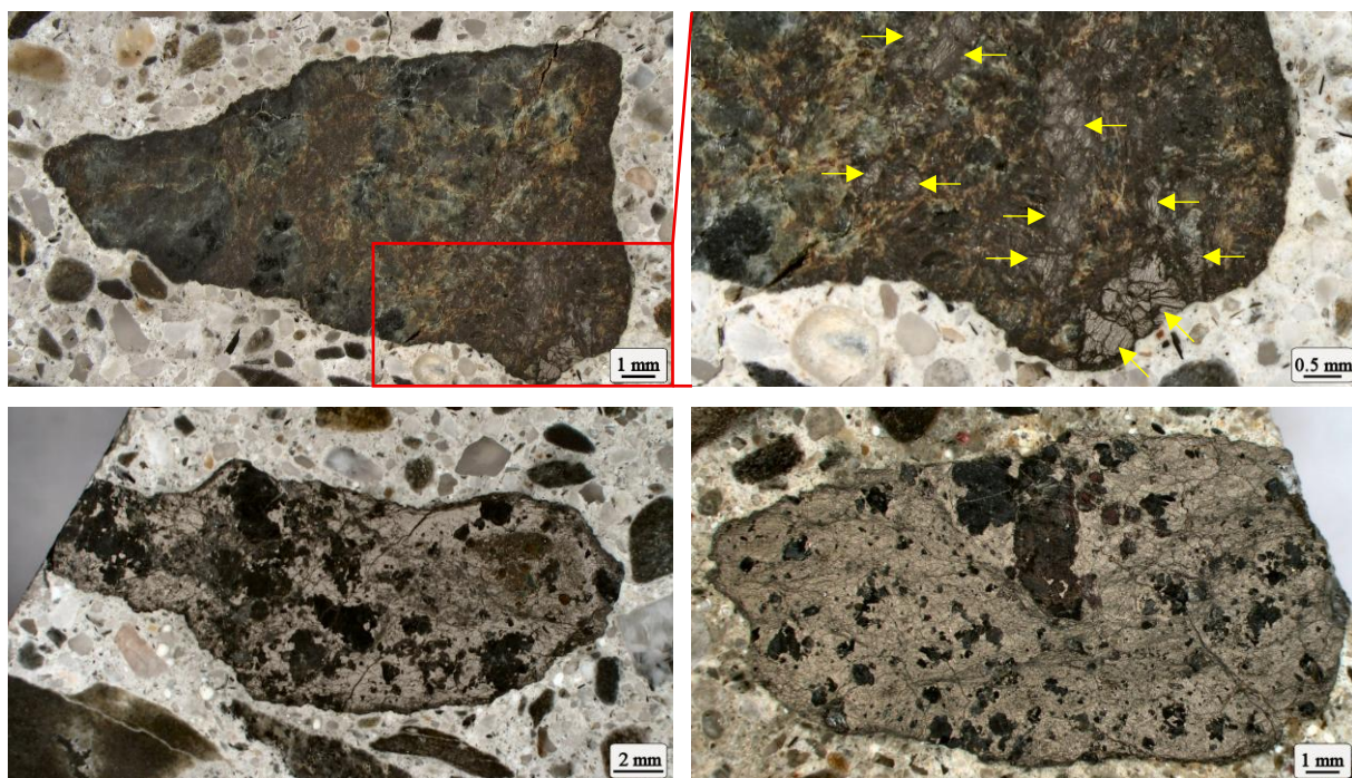
Figure 4: Representative examples of the reactive, pyrrhotite-bearing Dracut coarse aggregate particles. The upper photos show a chlorite schist particle with highly oxidized pyrrhotite (arrows), while the lower photos show particles comprised almost entirely of pyrrhotite.
