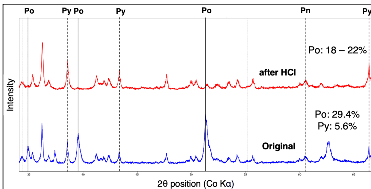
Figure 3.2: XRD diffractograms of sample MSK_4 before and after the initial HCl dissolution step. Characteristic pyrrhotite peaks disappear following the treatment, while other sulfide peaks remain. The Po content, ranging from 18% to 22%, was determined from calculations using the sulfur concentration obtained from the dissolved sample. Key: Po = pyrrhotite; Py = pyrite; Pn = pentlandite
