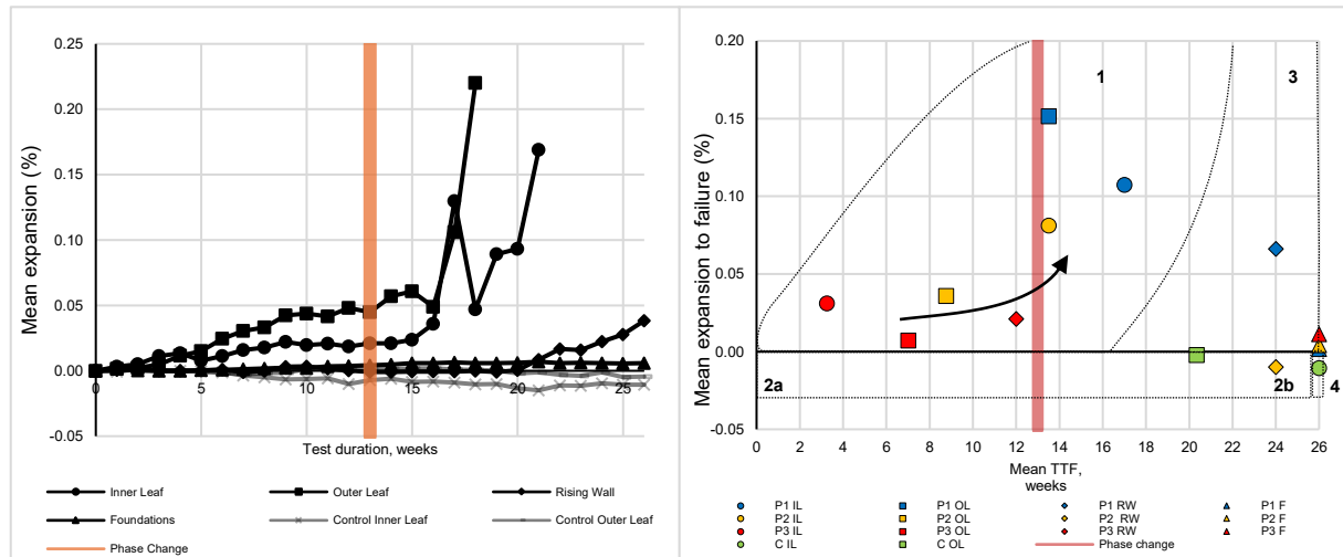
Figure 3.1 (left) Mean expansion of the test properties versus the control property, with the change of storage conditions marked at 13 weeks (red line). Figure 3.2 (right) Mean expansion at failure against time to failure exhibits approximate population areas 1 to 4, interpreted as: 1) expansive failures with greater expansion over time; 2) non-expansive failures related to initial condition or localised sample failures; 3) intact, still-expanding, typically late-stage expansive results; 4) intact samples that did not significantly expand. Note that some plots are obscured behind others. P1, P2, P3 F. A single P1 F 13-week TTF value was taken off test (non-failure for comparative reasons between phases 1 and 2) and is not included in mean TTF calculations. The arrow indicates the generalised progression of core expansion over time seen within population area 1 samples.
