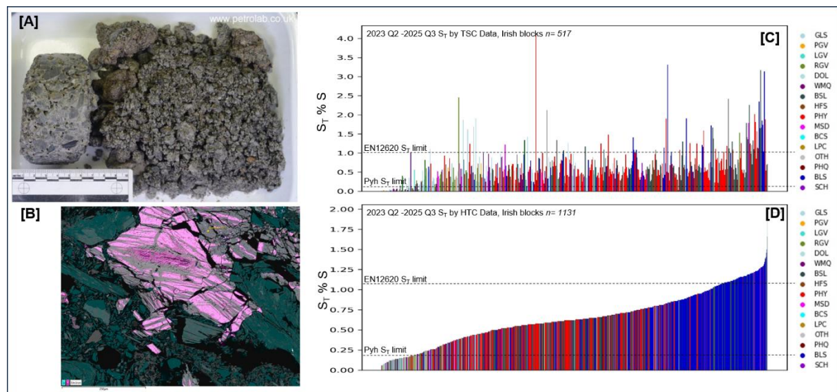
Figure 4.1: [A] Example PHY core [B] oxidised pyh in PHY aggregate [C] TSC determined S_T results coloured by lithology code and arranged by ascending HTC S% [D] HTC determined S_T results coloured by lithology code arranged by ascending HTC S%.
