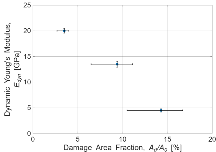
Figure 4.8: The dynamic Young's modulus (longitudinal mode) against the damage area fraction. Vertical error bars are plus/minus the standard deviation of the three, while horizontal error bars show the minimum and maximum of the damage area fraction from the four methods.
