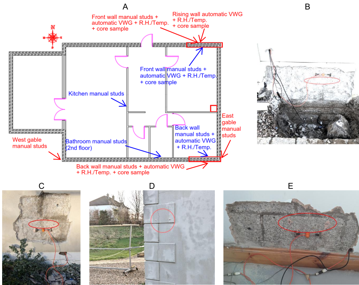
Figure 1.1: Selection of locations of monitoring and core samples within the selected concrete blocks (red circles show locations of manual expansion measurements with studs). A: Schematic of the monitoring and core sample locations, B: Exterior wall outer leaf and rising wall block below, front of house (facing north), C: Exterior wall outer leaf, back of house (facing south), D: Exterior wall outer leaf, east facing gable, E: Exterior wall inner leaf, back of house (facing south).
