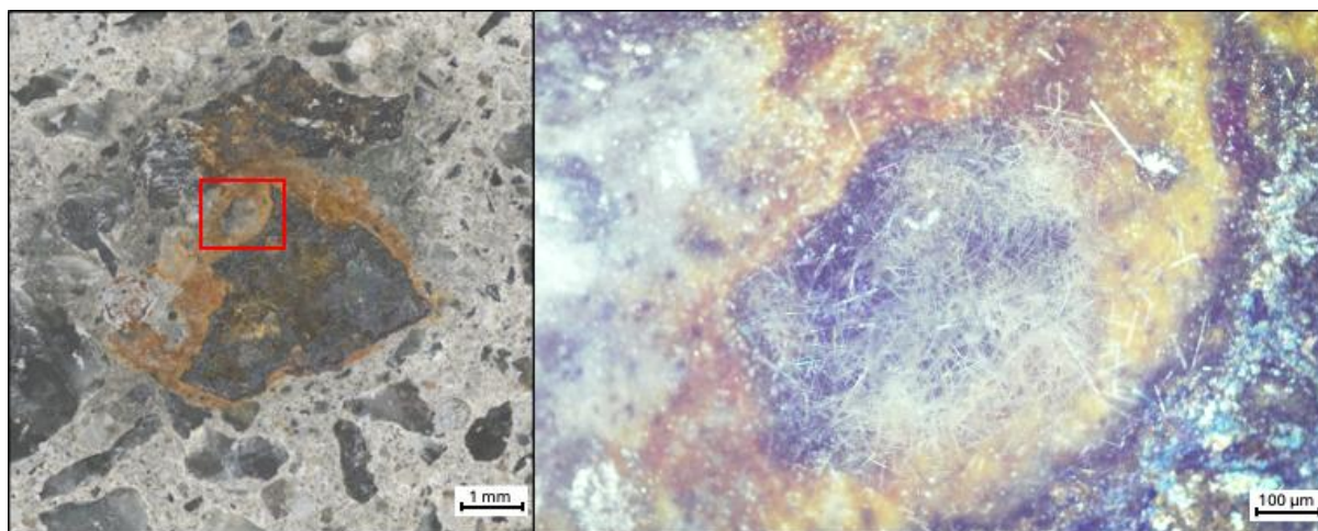
Figure 3.1: Sample P-2 (UV/ozone exposure) after three weeks. Left, staining and white mineral growth. Right, thin white needles can be seen growing into the cavity from the edges.
