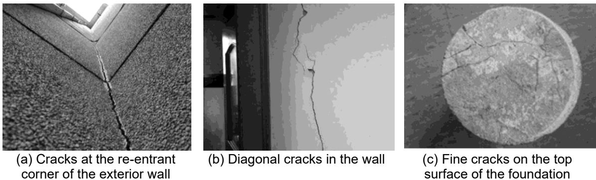
Figure 2.3: Deterioration characteristics of masonry residential building 2 [2]
