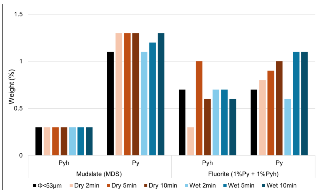
Figure 3.2. Sulfide variation in MDS (natural aggregate) and Fl+1% Py+1% Pyh (synthetic mixtures).
