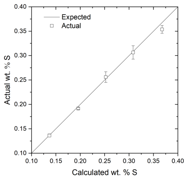
Figure 3.2. Results of component mixture combustion vs. calculated values, based on results of individual RM components. Error bars represent relative standard deviation.
