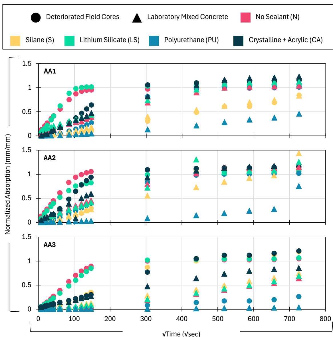
Figure 3.1. Initial and secondary absorption for different sealants. The uncertainty (relative standard deviation) for absorption value series was 5% for the field cores and was 3% for the lab cores.
