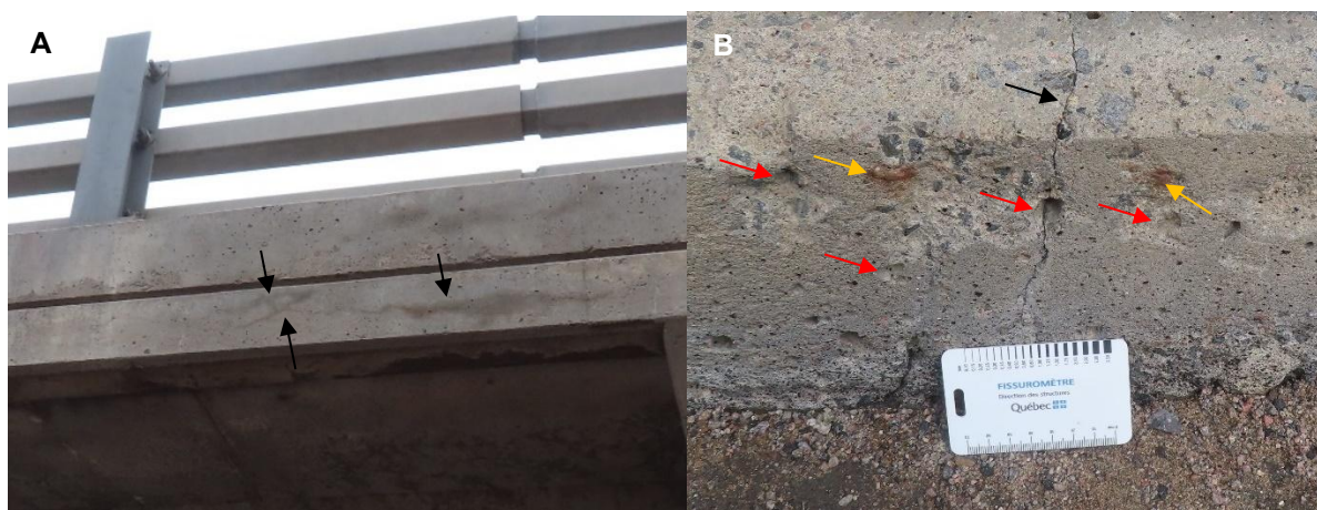
Figure 4.2: A) Longitudinal cracks on the exterior side of the deck. B) Vertical crack (black arrow), rust stains (orange arrows) and pop-outs (red arrows) on the curb.
