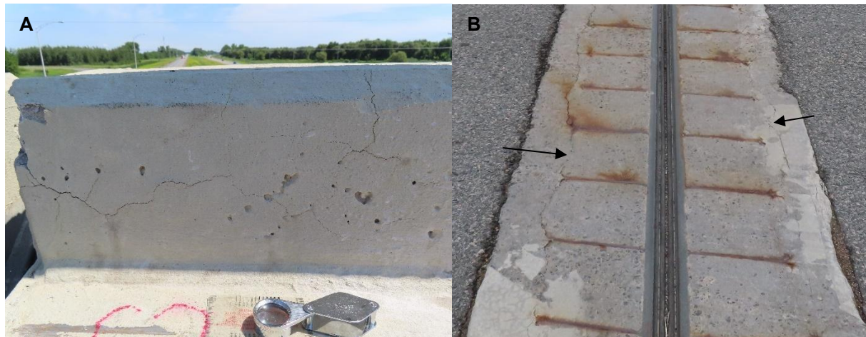
Figure 4.1: A) Polygonal cracking pattern on thin repairs on the curb. B) Large crack at the end of the steel plates of the expansion joint.
