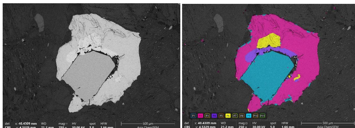
Figure 2.4: Backscattered electron (BSE) image of reflected light image field of view shown in figure 2.1A (left) and EDS x-ray phase map (right) depicting different iron-sulfide mineral phases detected through differentiation of statistically significant spectra.
