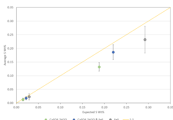
Figure 2.1.2.1: HTC Results of Standards
