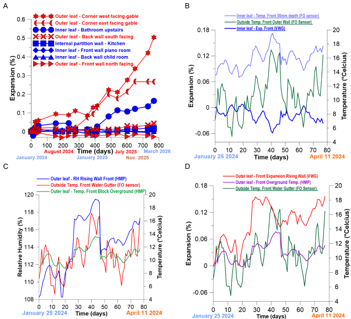
Figure 3.3: Graphs of expansion, temperature and R.H. monitoring A: Manual expansion measurements over almost two years, B: Inner leaf and outside temperature data, along with VWG (automatic) expansion measurements (first three months), C: Outer leaf and outside temperature data, along with rising wall R.H. (first three months), D: Outer leaf and outside temperature data, along with VWG rising wall expansion (first three months).
