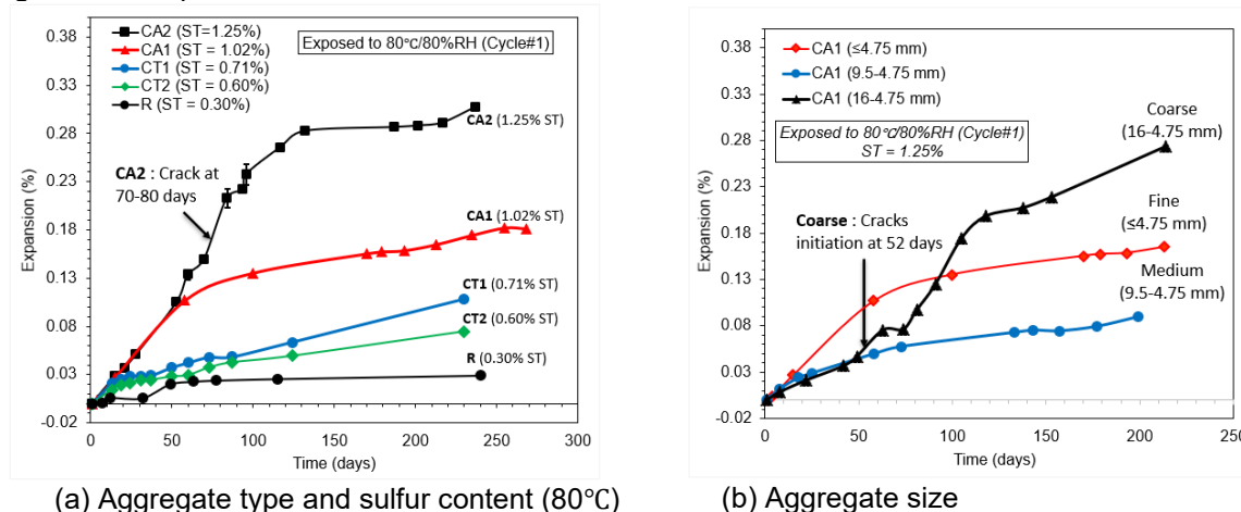
Figure 3.2. Effect of sulfur content and aggregates size on the expansion of sulfide-bearing aggregate.
