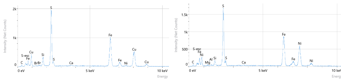
Figure 2.5: Individual phases of x-ray map separated and accompanied by associated spectra.
